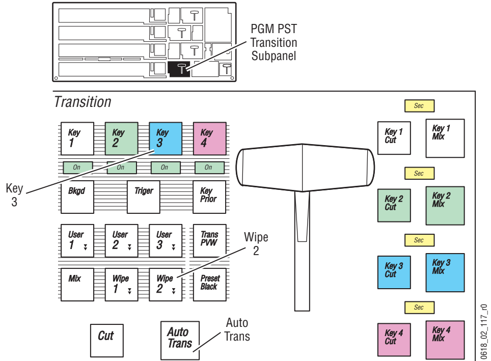
Figure 252. PGM PST Transition Subpanel
