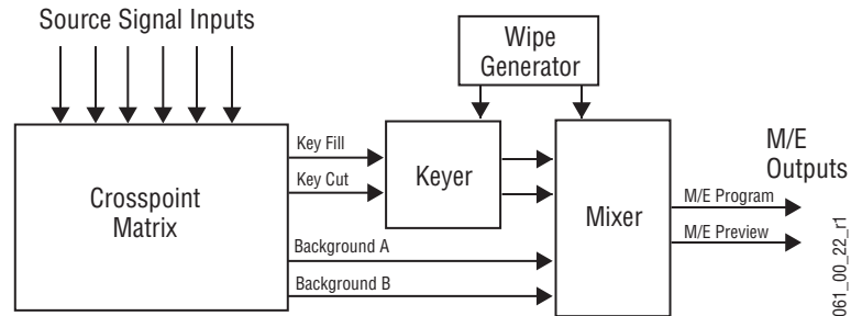
Figure 49. Simplified Mix Effects (M/E) Subsystem
