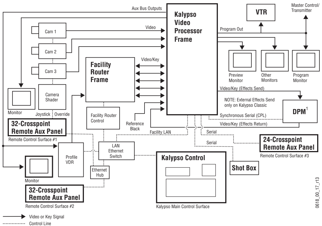
Figure 39. Basic Live Production Studio System Configuration Example
