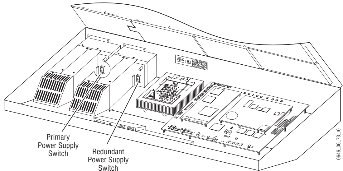
Figure 118. Main Panel, Lid Open
