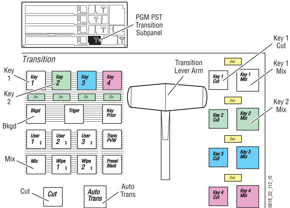
Figure 247. PGM PST Transition Subpanel, Keyer Transitions
