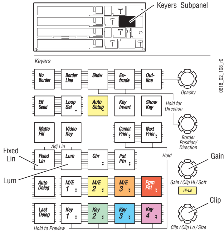
Figure 243. Keyers Subpanel, Basic Keying Controls
