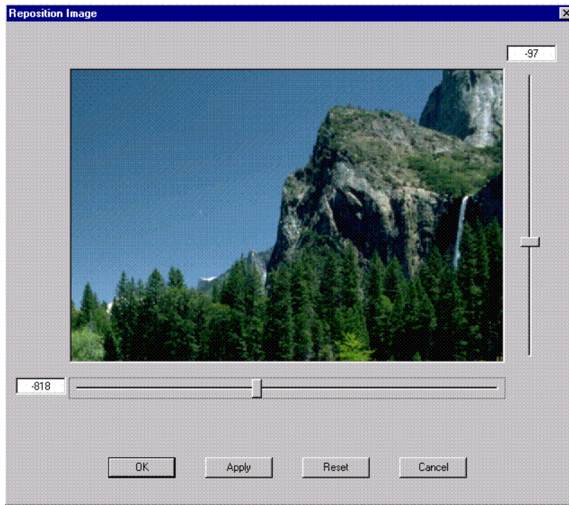
Figure 291. Repositioned Image
