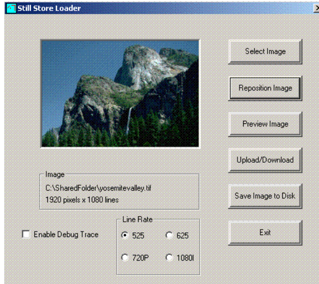
Figure 288. Opened Image
