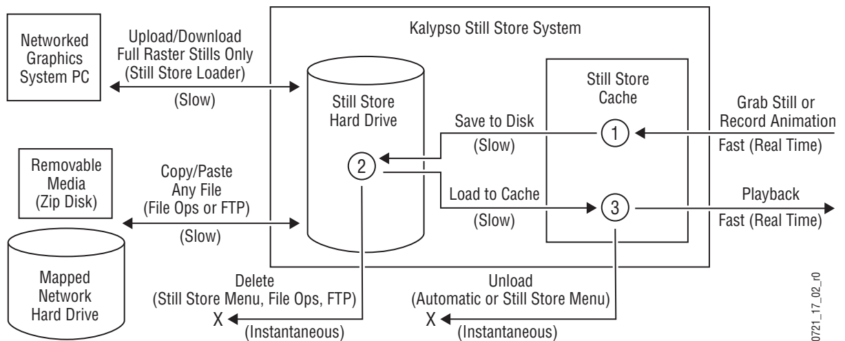
Figure 188. Kalypso Still Store System
