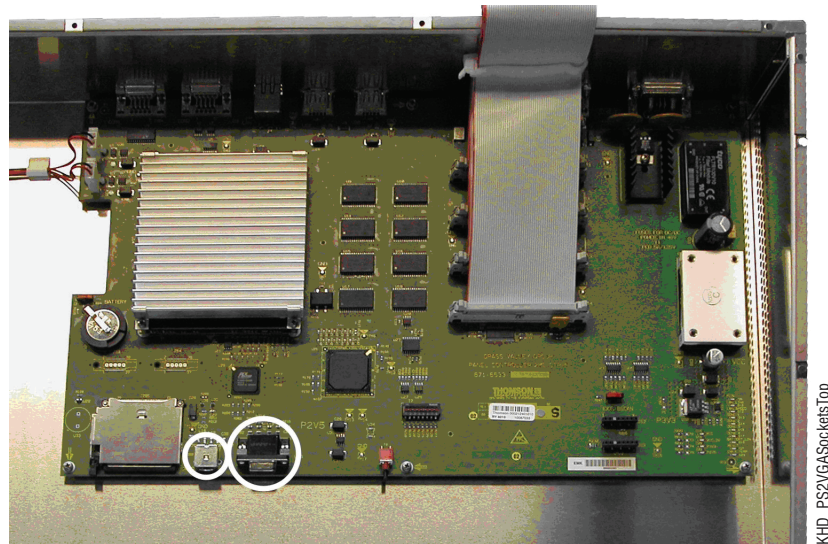
Figure 113. Top View PS/2 and VGA Sockets on the Kayak HD Panel
