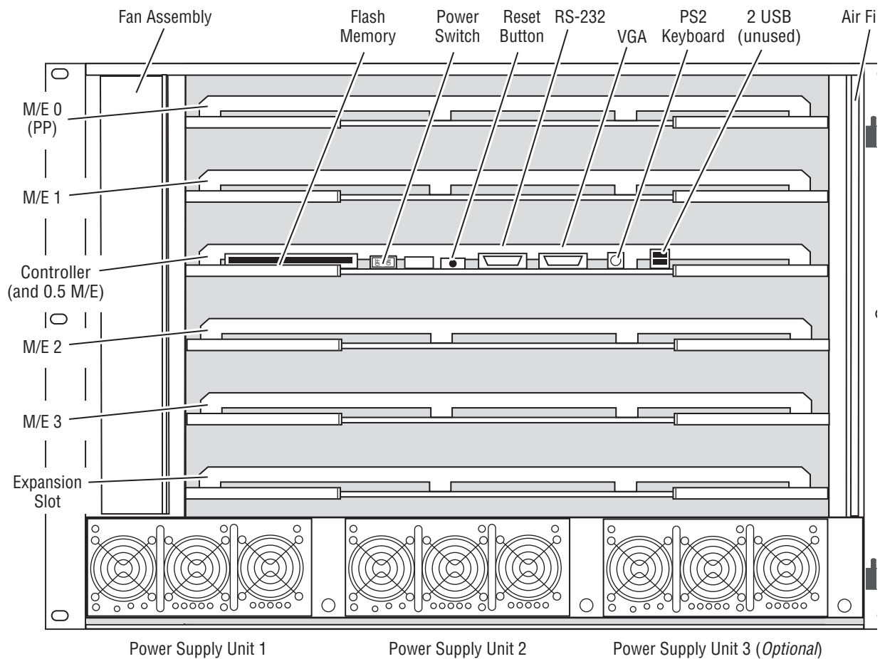
Figure 21. Kayak HD 8RU Frame, Front View with Door Removed
