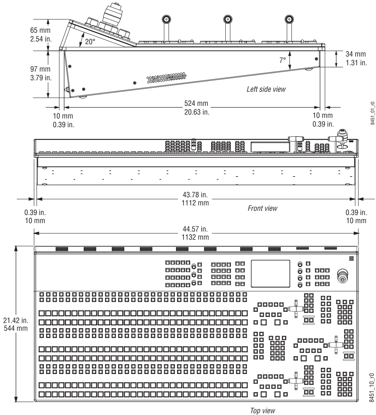
Figure 29. Kayak HD 250C, 250, and 300 Control Panel Dimensions
