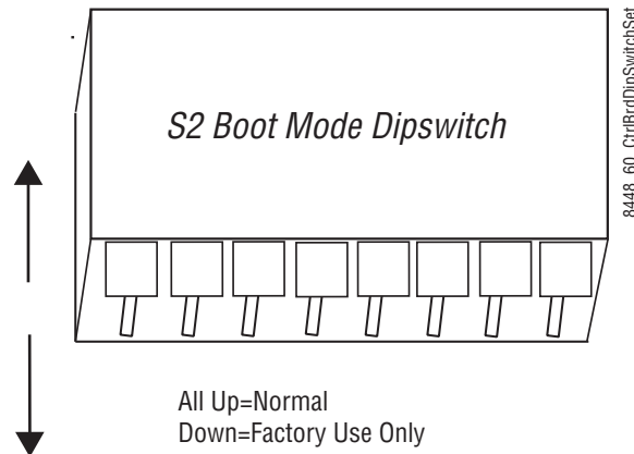
Figure 107. Kayak Control Processor Board - S2 Boot Mode Dipswitch Setting
