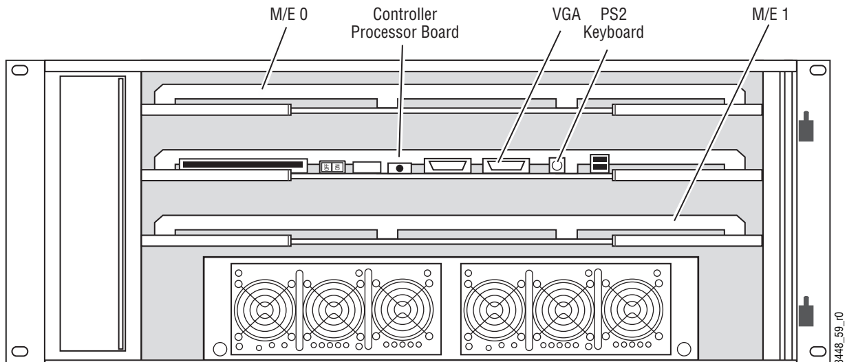
Figure 112. Side View PS/2 and VGA Sockets on the Kayak HD Controller Processor Board
