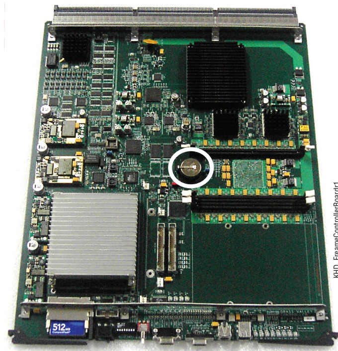
Figure 108. Kayak HD Frame Controller Board with Battery in center of board
