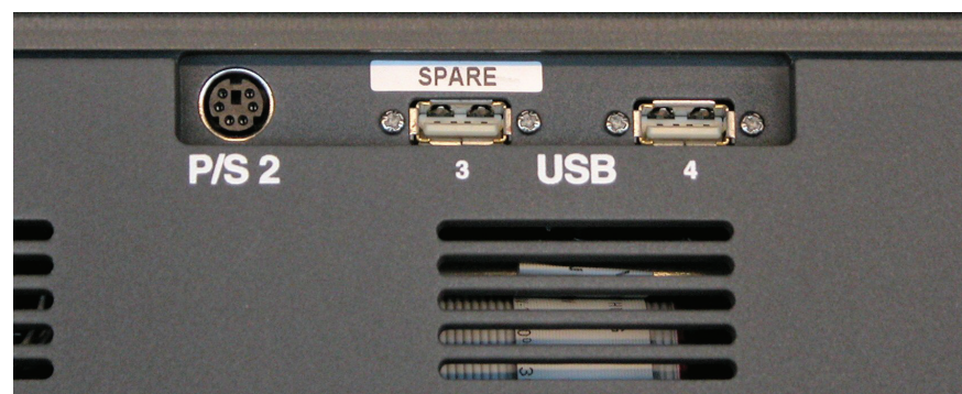
Figure 32. Kayak HD Connectors Top Rear Control Panel
