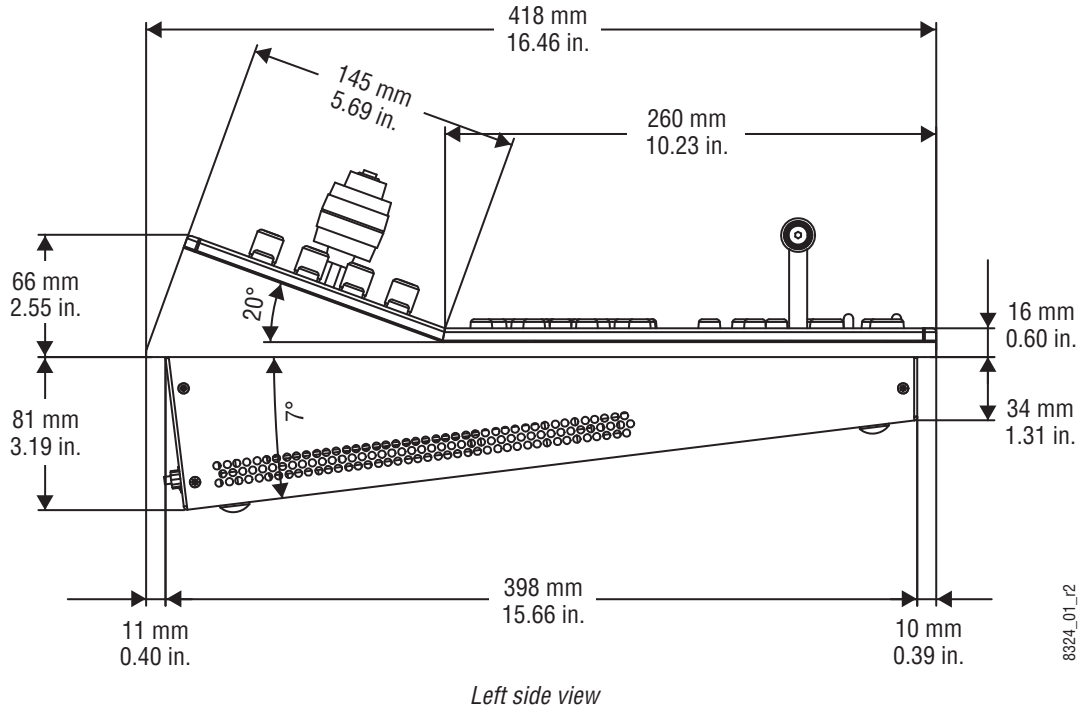
Figure 25. Kayak HD 100C Control Panel Dimensions 1 of 2
