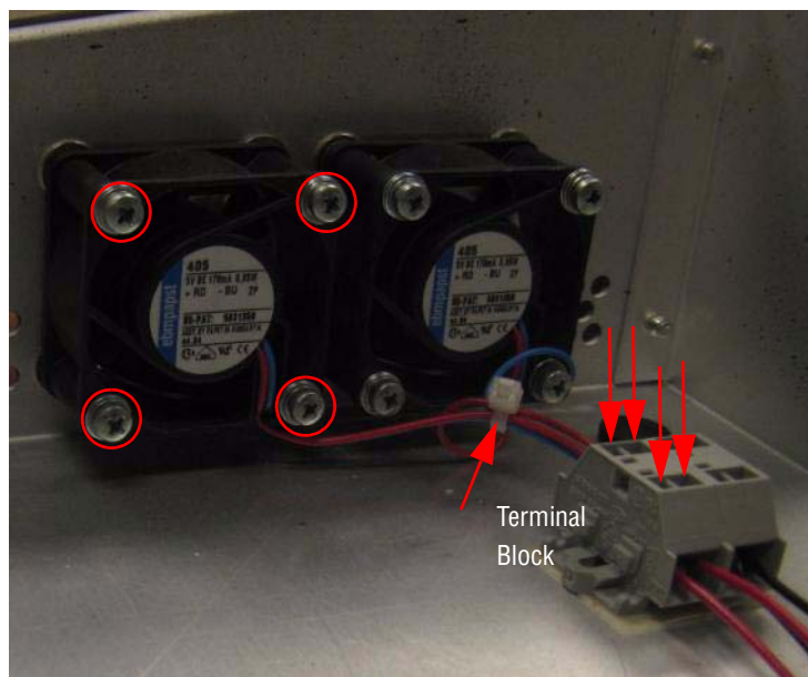
Figure 141. Kayak 2ME Control Panel Fans—Replace Fans
