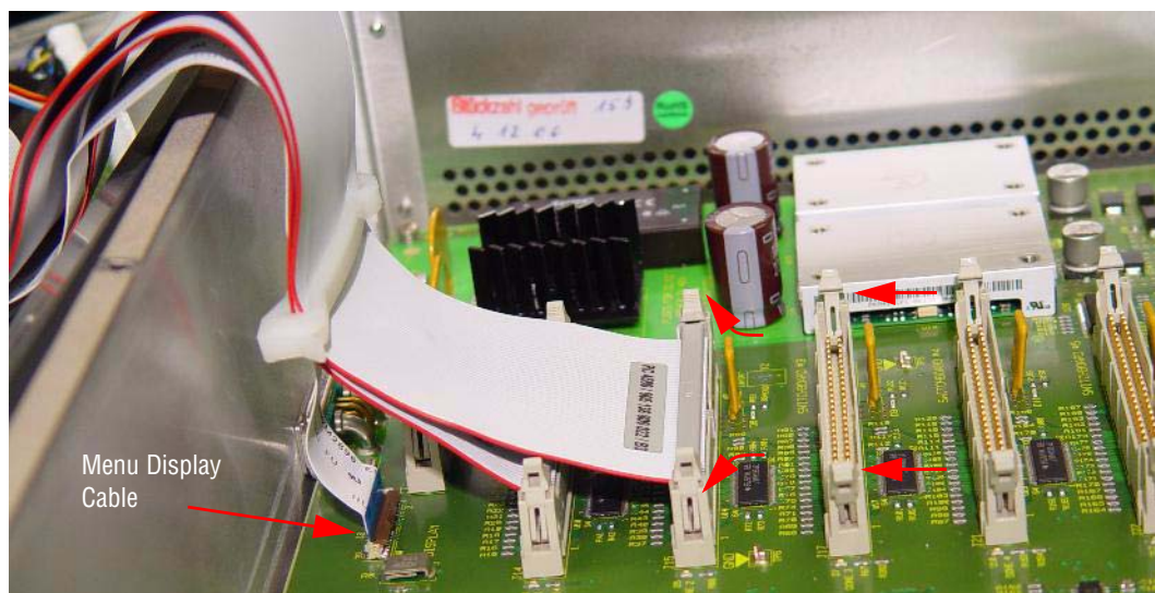
Figure 135. Kayak Control Panel Ribbon Cable Harness—Disconnecting the Ribbon Cable Harness
