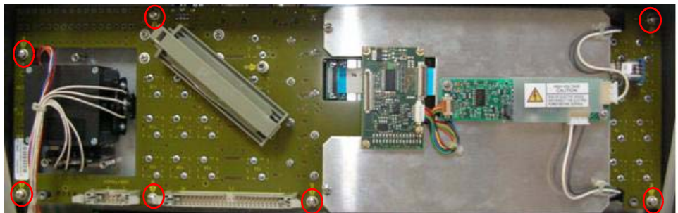
Figure 128. Menu Display Board—Board to Enclosure Screw Removal
