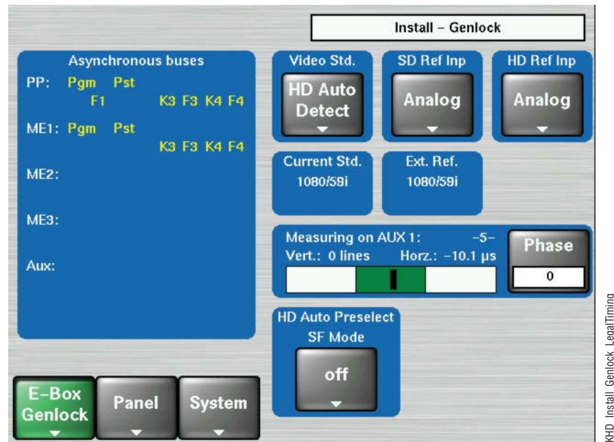
Figure 43. Genlock Menu
