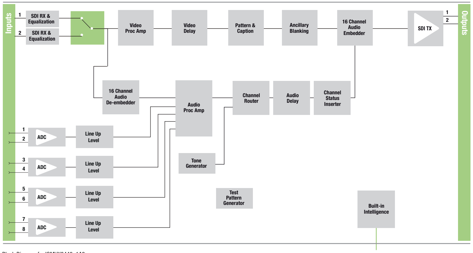
Block Diagram for IQMUX3449-1A3
