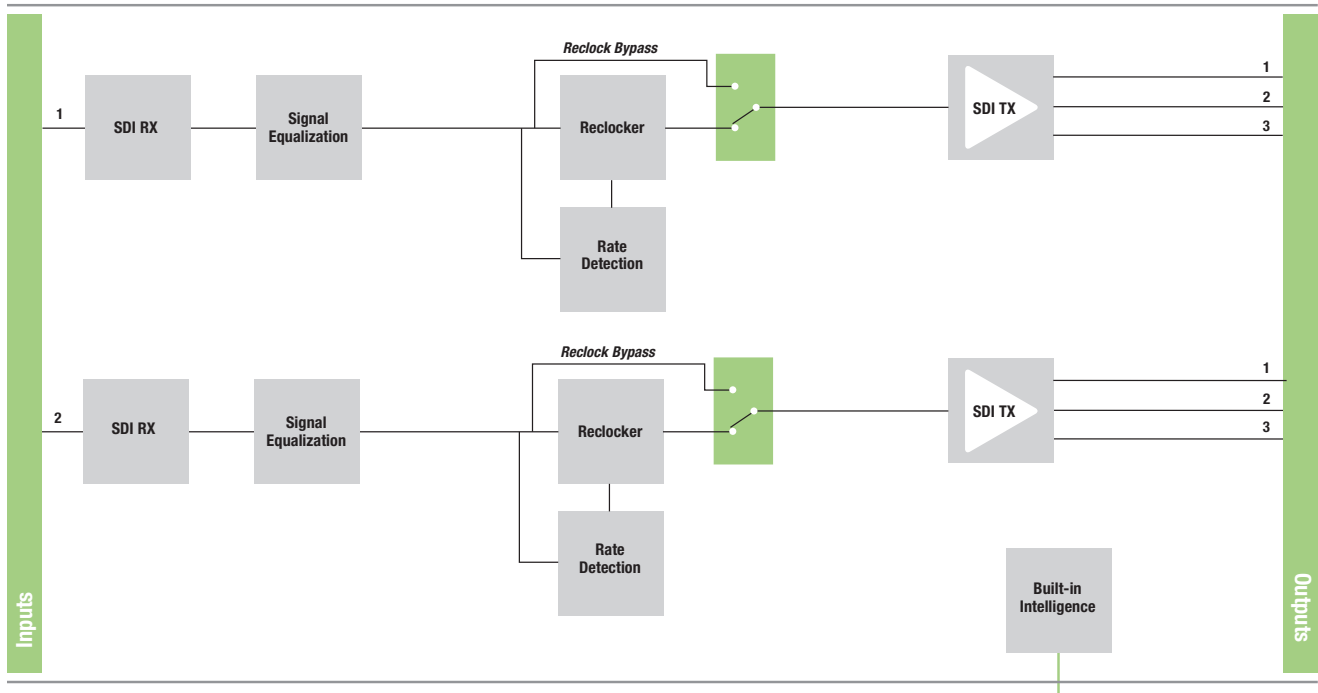
Block Diagram for IQSDA3047-1B3
