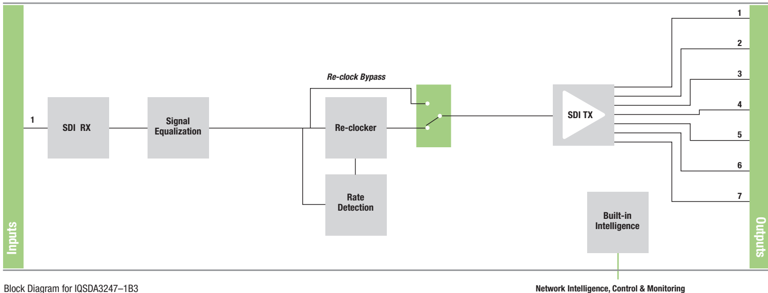
Block Diagram for IQSDA3247-1B3
