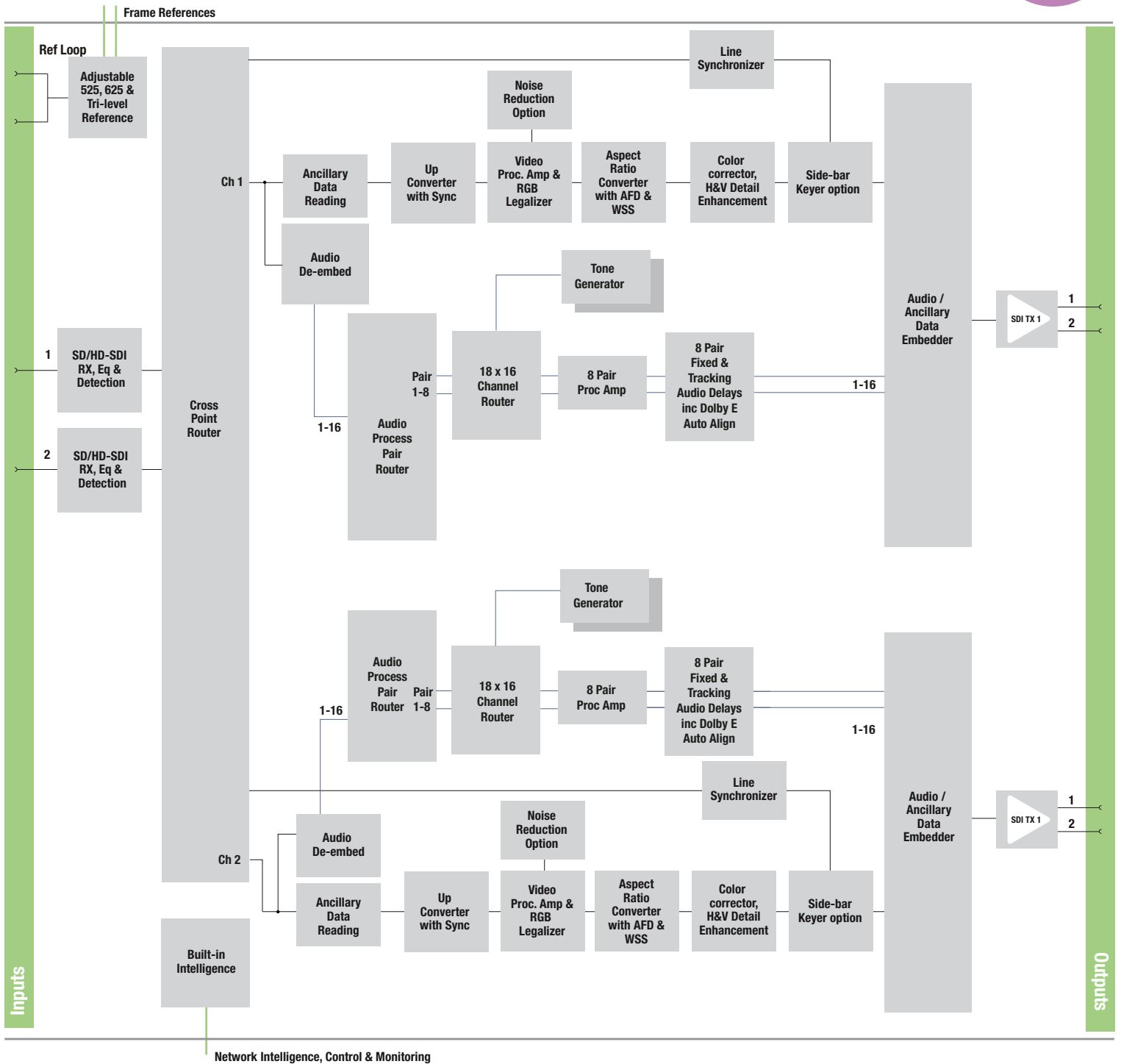
Block Diagram for IQUPC31 Range.
