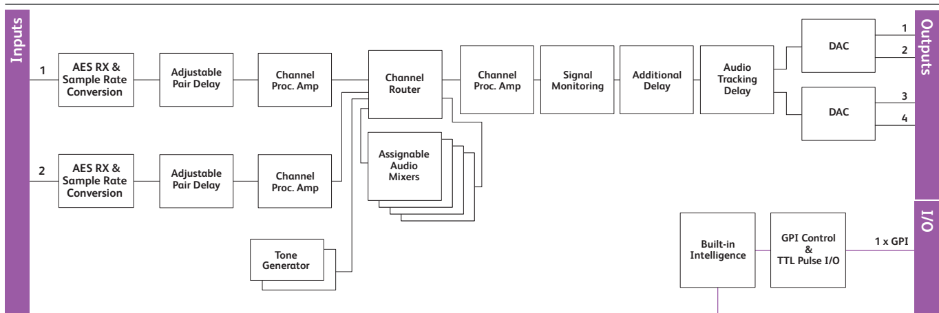
Block Diagram for IQDAA0015-1A
