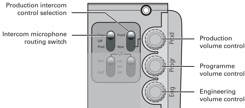
Figure 5-13. Intercom controls
