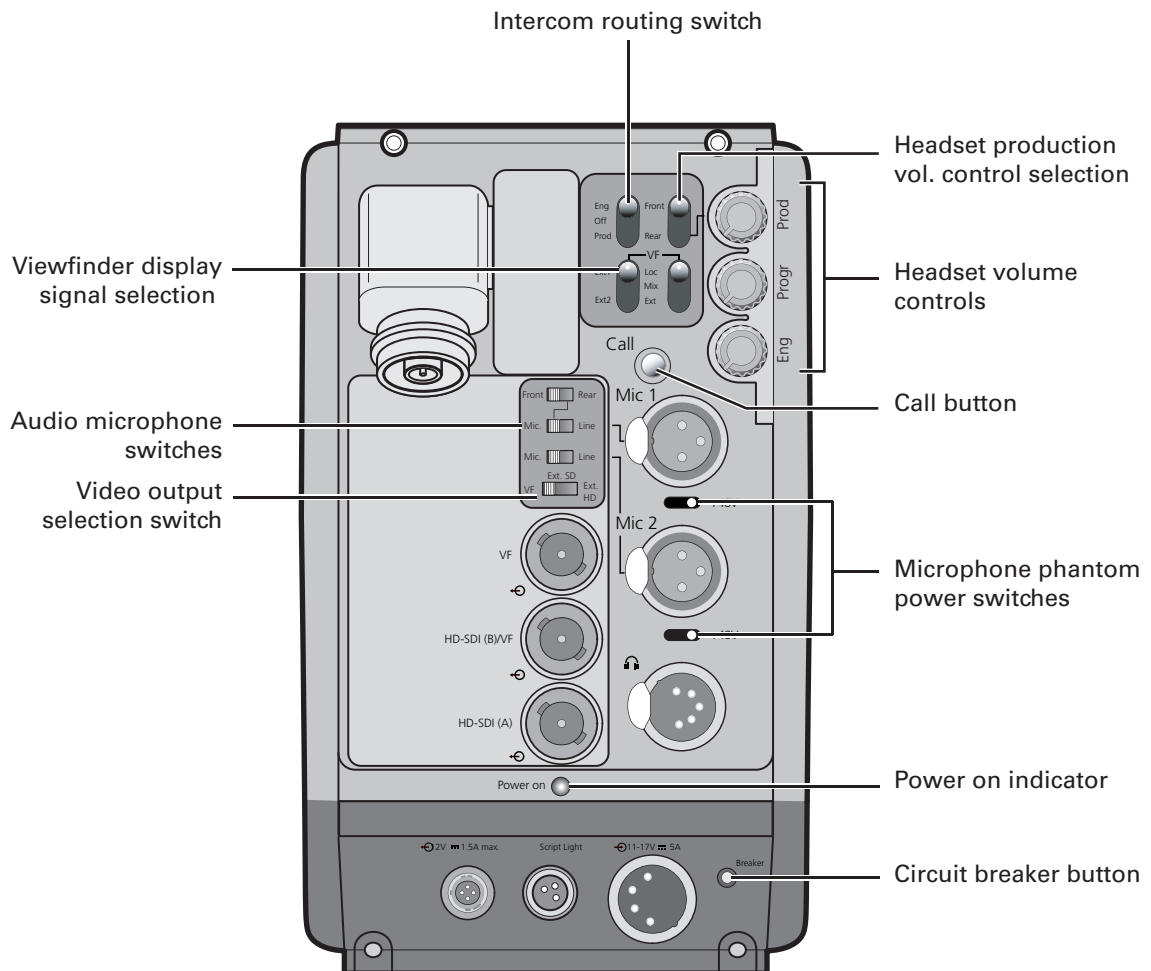
Figure 5-1. Rear controls
