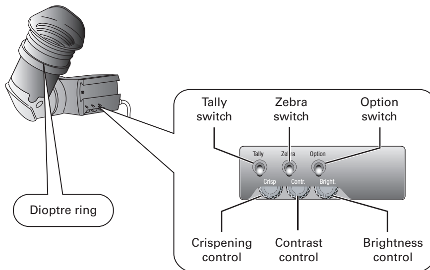
Figure 5-5. Viewfinder controls
