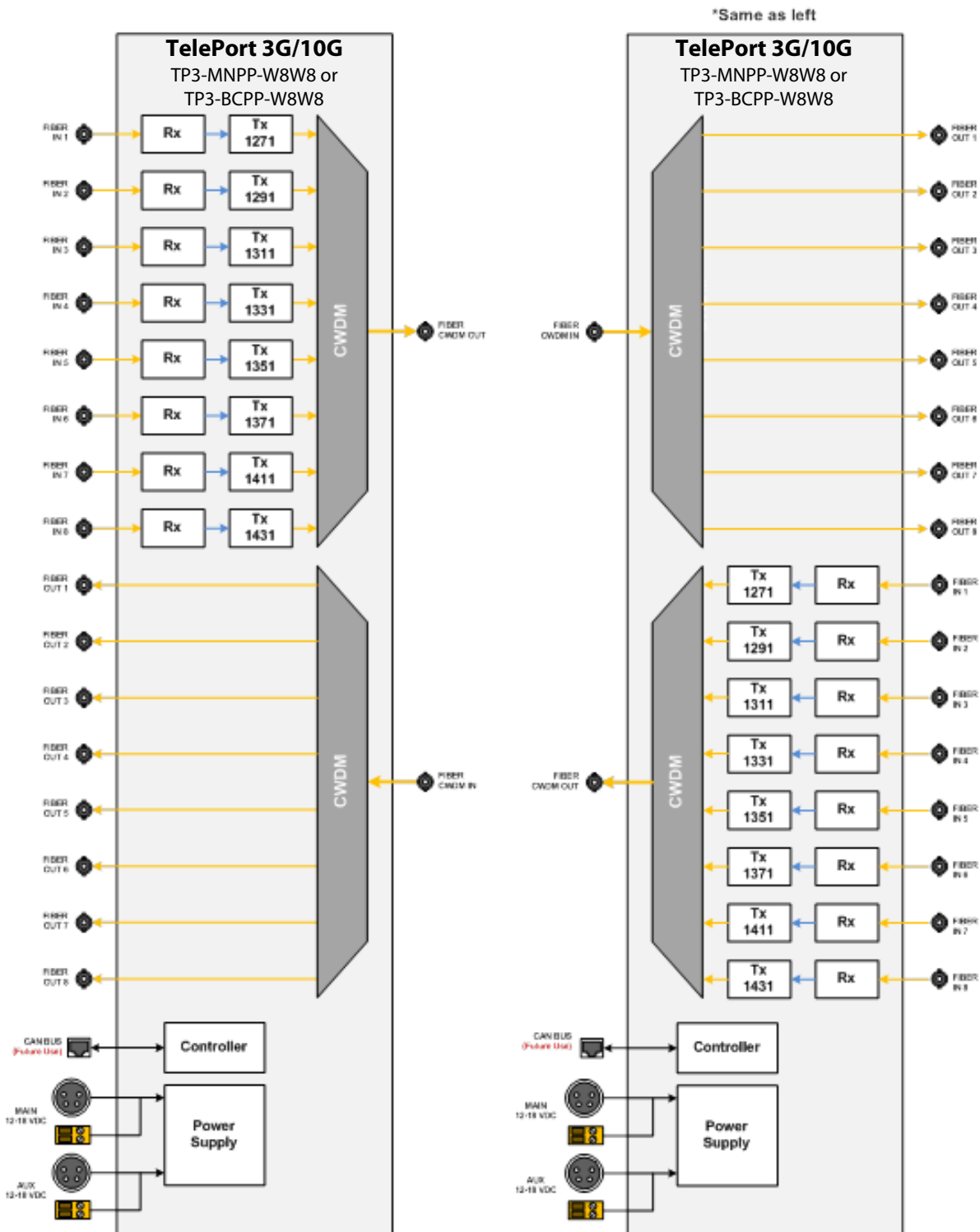
Fig. 2-1: 8x8 Channels TelePort 3G/10G on 2 Fibers Block Diagram
