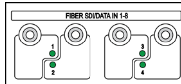
Fig. 3-7: 4 SDI/DATA In ST Connectors
