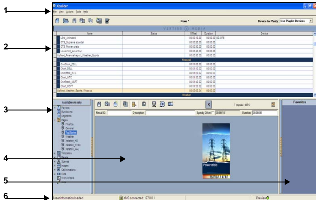
Fig. 2-1: Xbuilder interface
