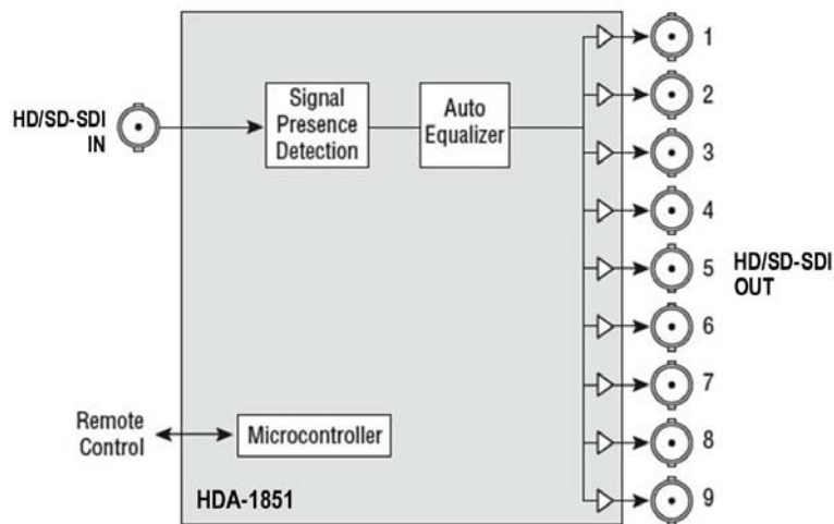
Figure 1.1 Functional block diagram of the HDA-1851
