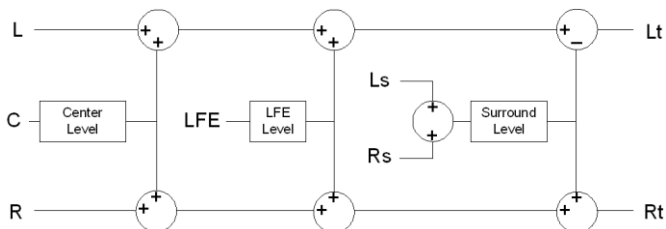
Figure 5.17 LtRt Surround Sound downmixer
