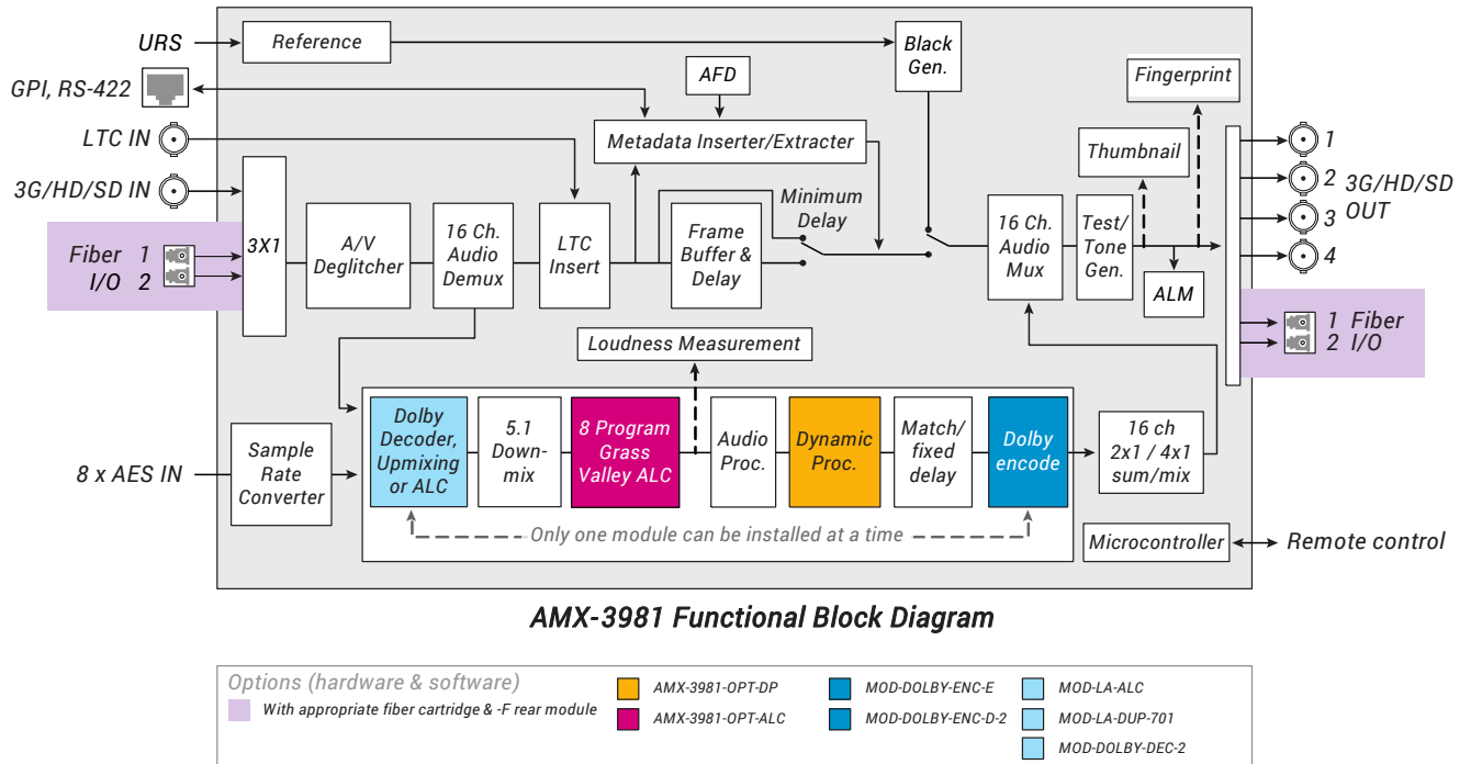
Figure 1.1 AMX-3981 Functional Block Diagram
