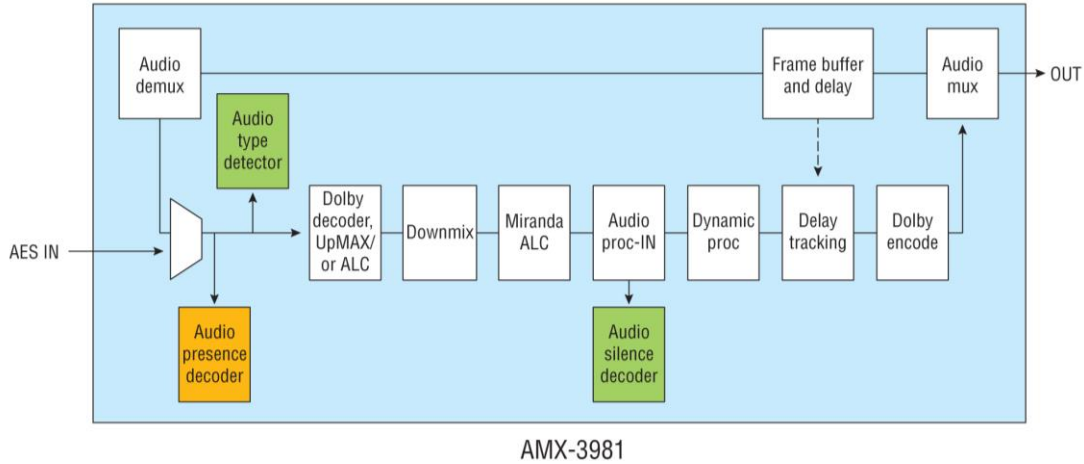
Figure 5.59 Relative position of audio presence and type detectors
