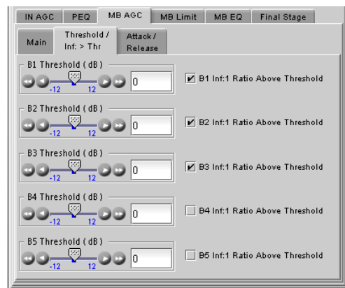
Figure 6.15 ALC - MB AGC - Threshold
