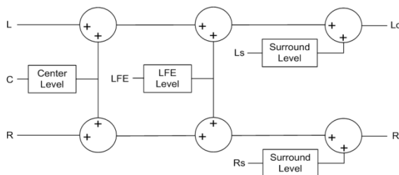
Figure 5.18 LoRo Stereo downmixer
