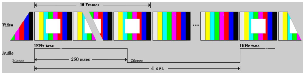
Figure 5.51 Lip Sync test signal appearance and timing
