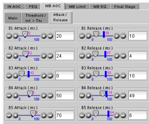
Figure 6.16 ALC - MB-AGC - Attack/Release
