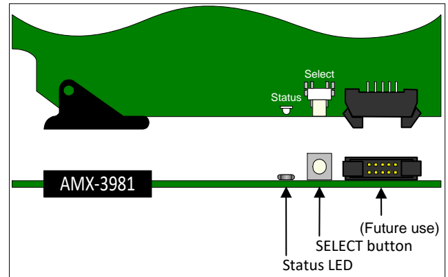
Figure 1.2 Front card-edge layout
