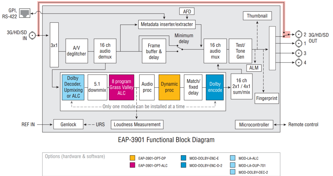
Figure 1.1 EAP-3901 Functional Block Diagram
