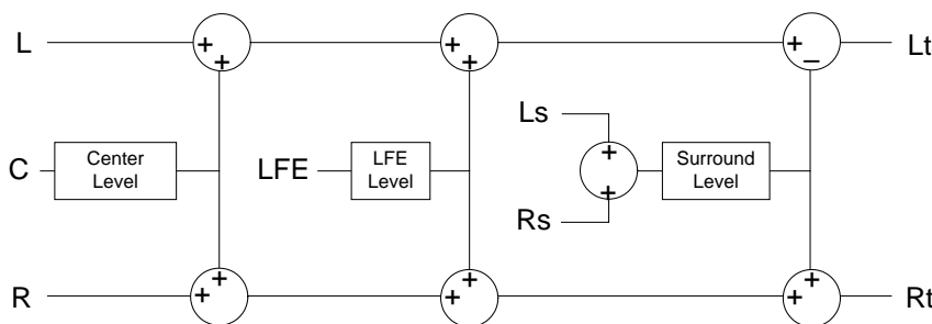
Figure 5-15 LtRt Surround Sound Downmixer
