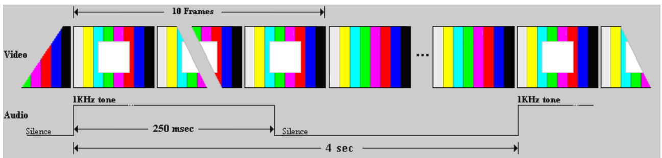
Figure 5-47 Lip Sync test signal appearance and timing
