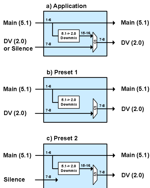
Figure 5.56 Application for automatic preset recall
