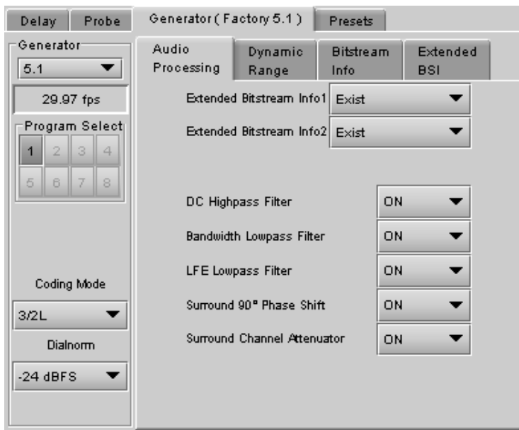
Figure 5-28 [Config] → [Generator] → [Audio Processing]
