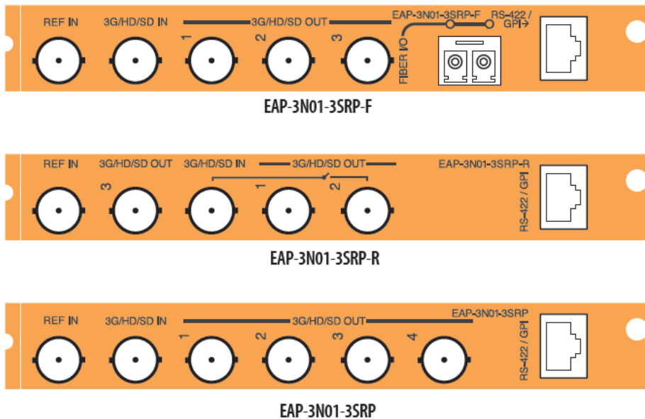
Figure 2-1 EAP-3901 rear panels
