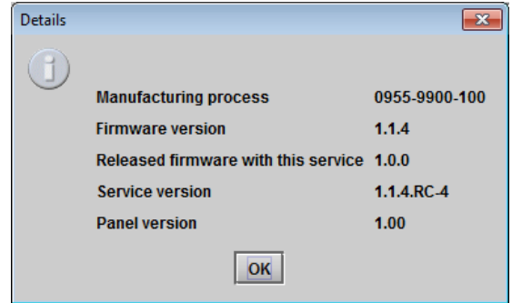
Figure 3.40 Details window
