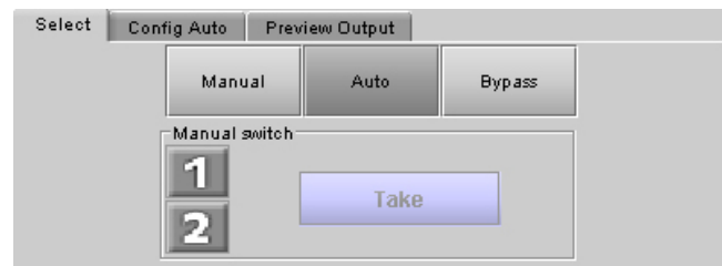
Figure 3.6 Auto Mode
