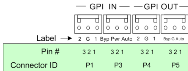
Figure 2.3 GPI Connectors
