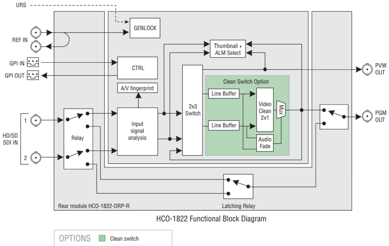
Figure 1.1 Functional block diagram HCO-1822
