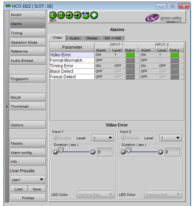
Figure 3.9 Alarms panel
