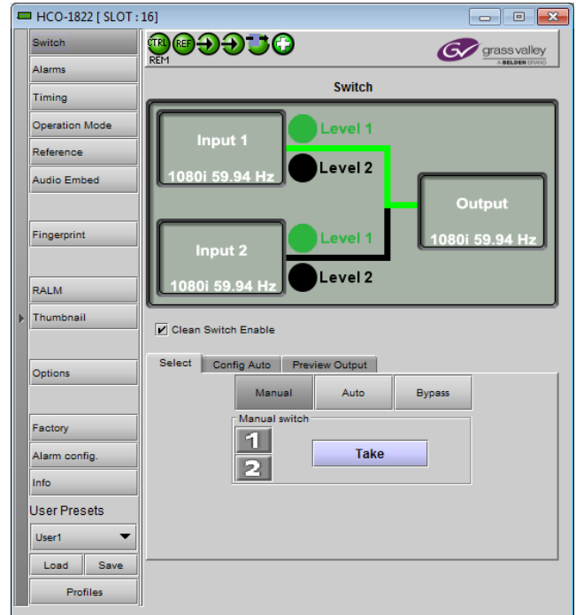
Figure 3.4 Switch panel
