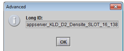
Figure 3.41 Advanced window
