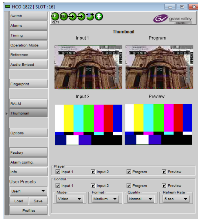
Figure 3.32 Thumbnail Panel
