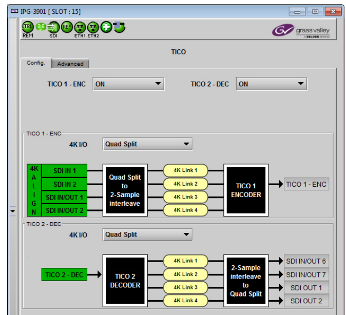
Figure 5-10 TICO panel - Config tab
