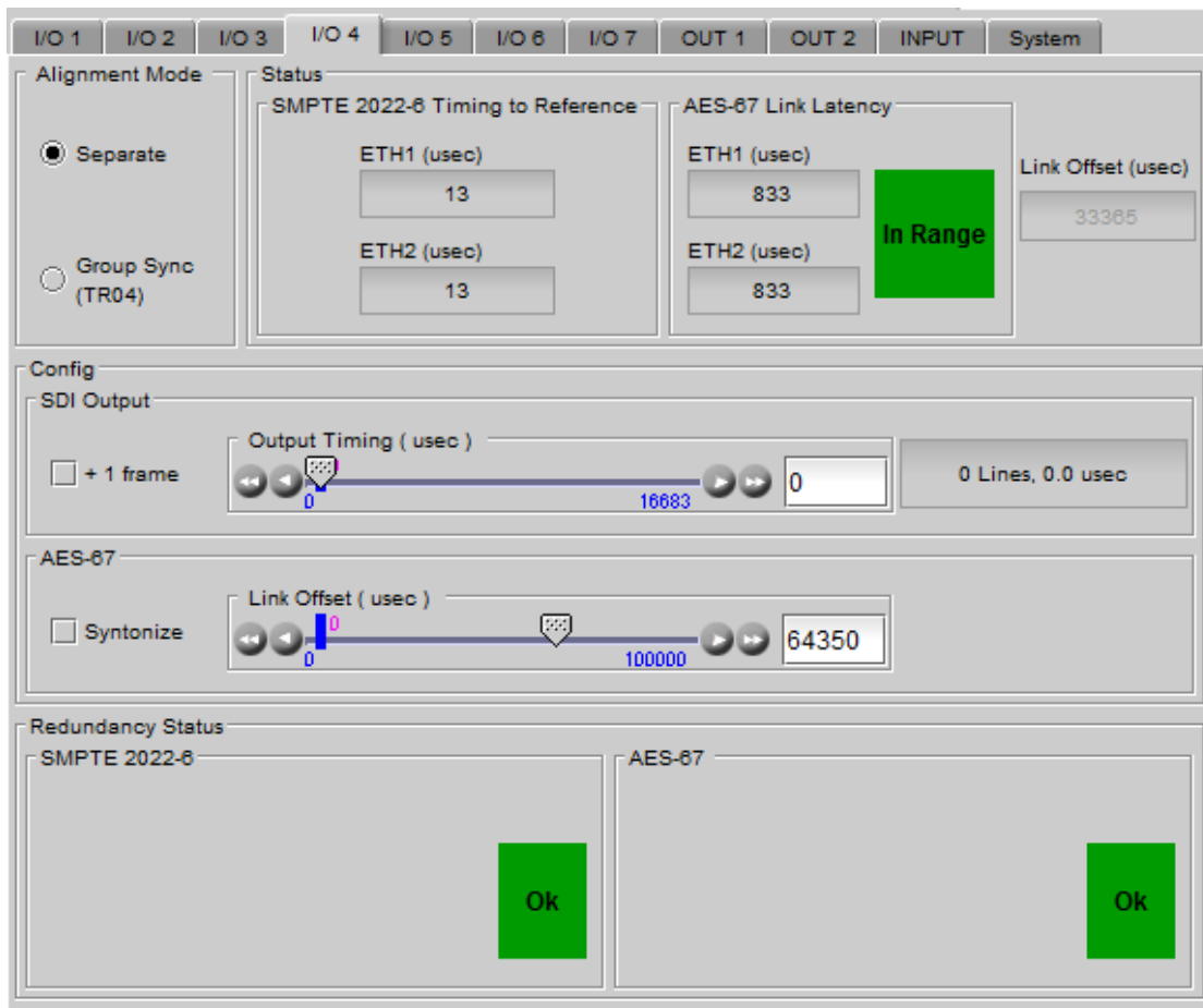
Figure 5-4 Gateway panel - lower portion – SDI output configuration
