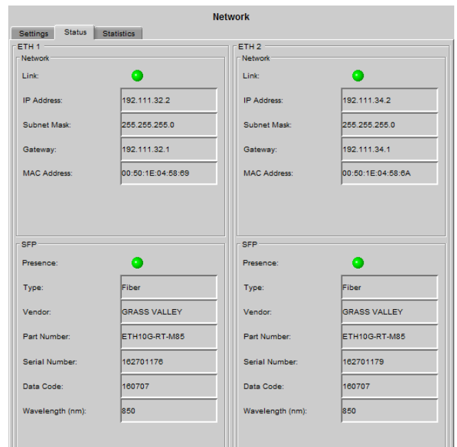
Figure 5-8 Network panel – Status tab
