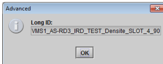
Figure 3.48 Advanced window
