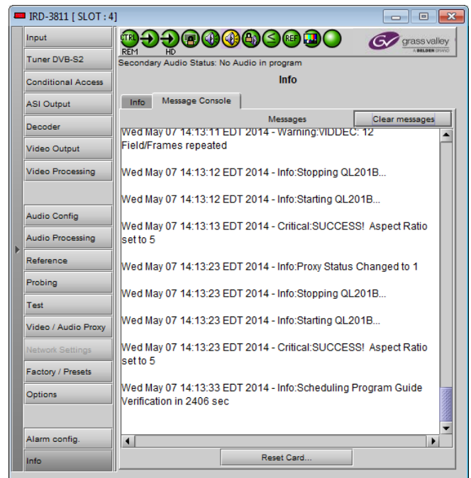
Figure 3.50 Message Console
