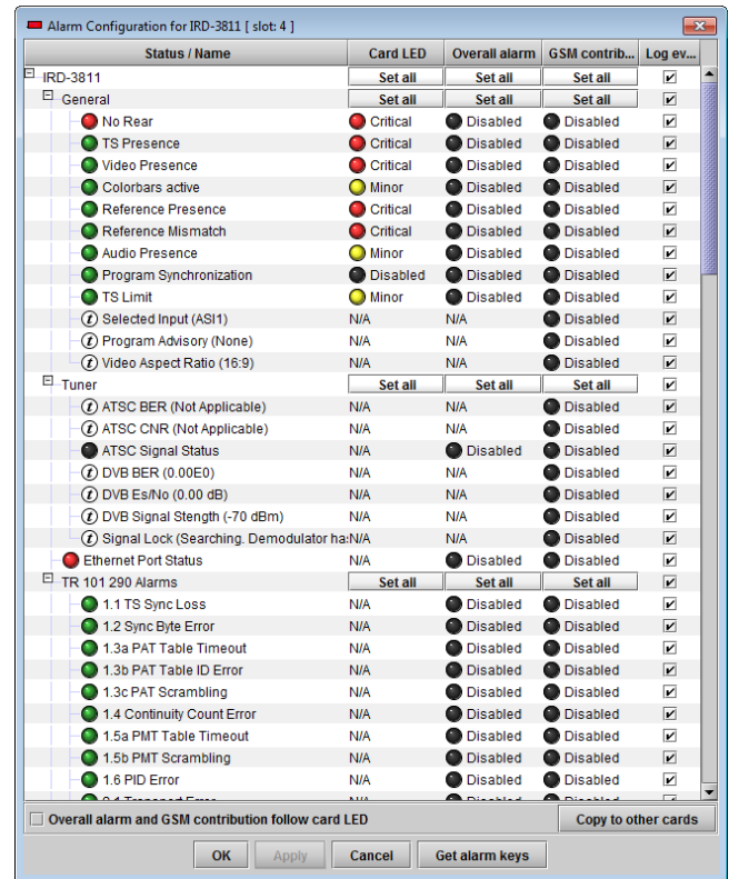
Figure 3.42 Alarm Configuration Panel
