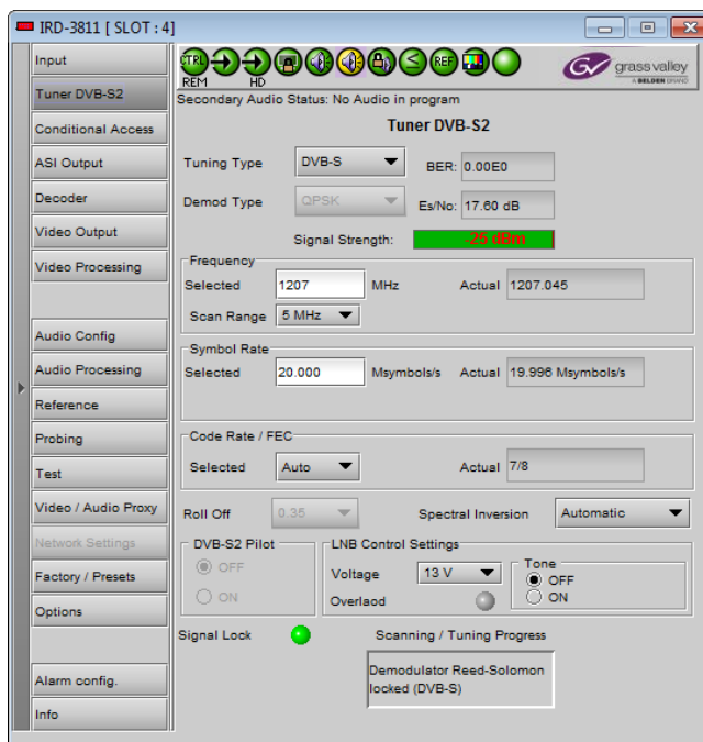
Figure 3.5 Tuner DVB-S2 panel
