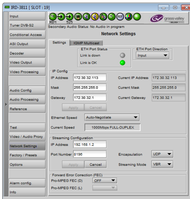
Figure 3.30 Network Settings panel – Settings tab
