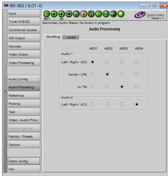
Figure 3.18 Audio Processing – Shuffling tab
