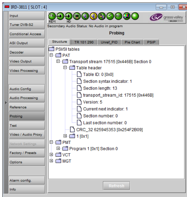
Figure 3.21 Probing panel – Structure tab
