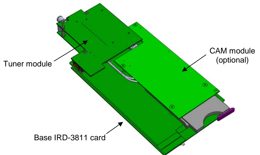
Figure 1.3 IRD-3811 physical layout
