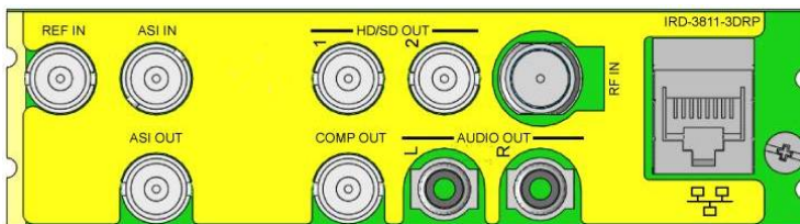
Figure 2.1 IRD-3811-3DRP Rear Panel for the IRD-3811
