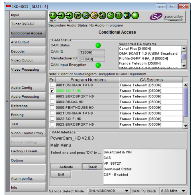
Figure 3.6 Conditional Access panel
