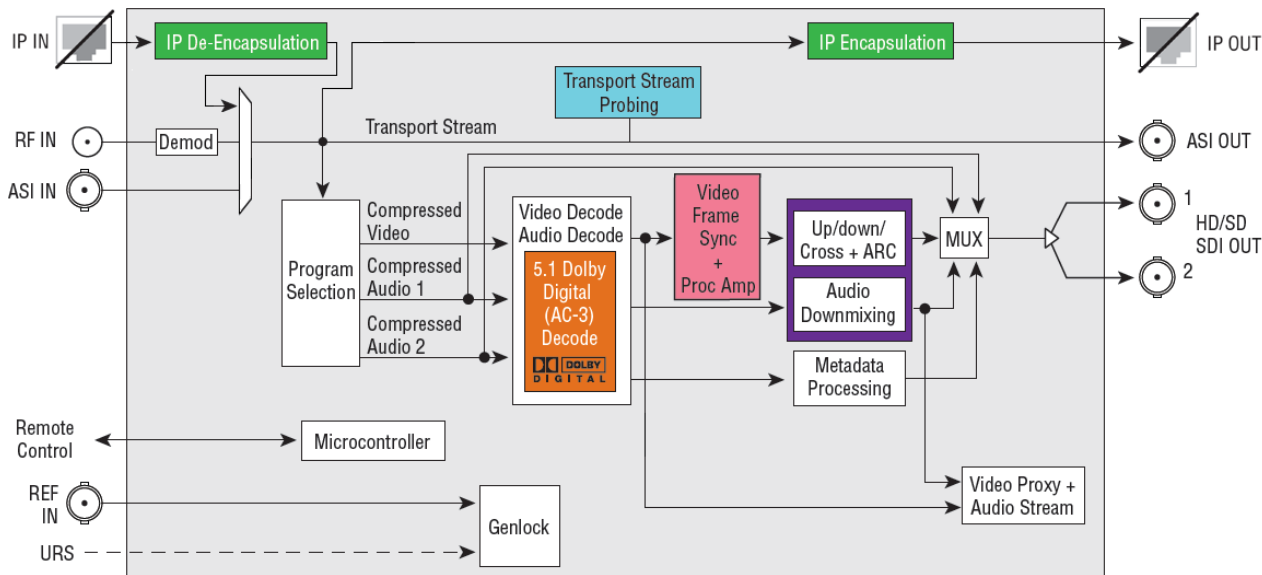
IRD-3811-VQ & IRD-3811-DVB-S2 Functional Block Diagram
