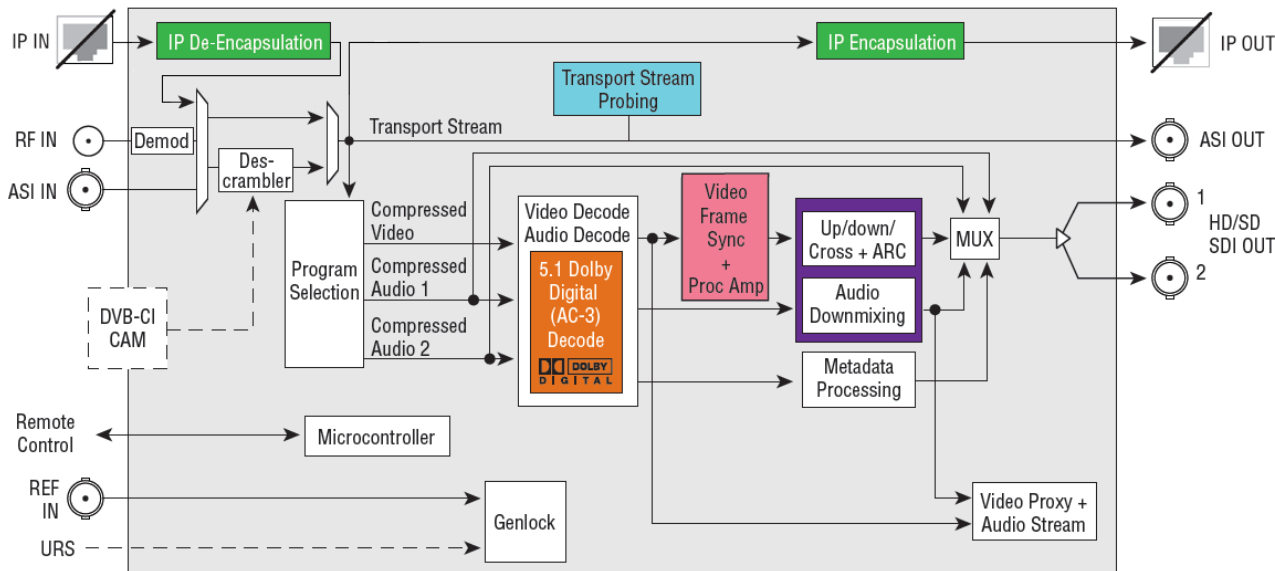
IRD-3811-VQ-CI & IRD-3811-DVB-S2-CI Functional Block Diagram
