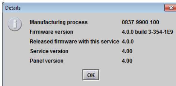
Figure 3.47 Details window
