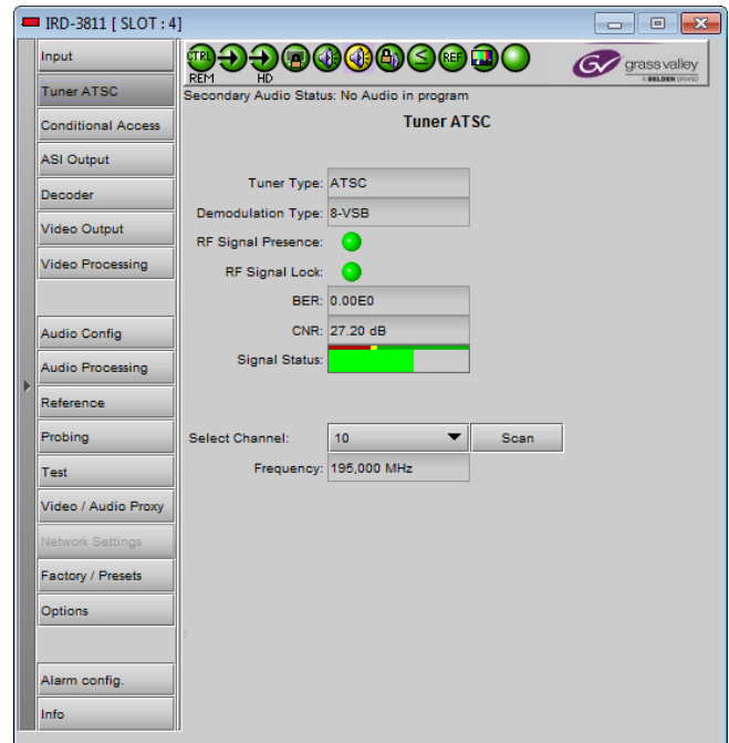
Figure 3.4 Tuner ATSC panel
