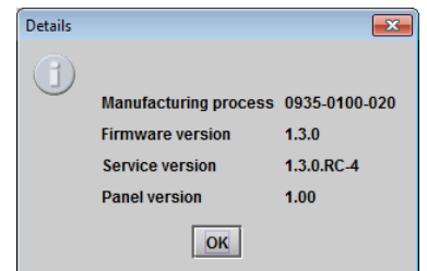
Figure 5-23 Details window
