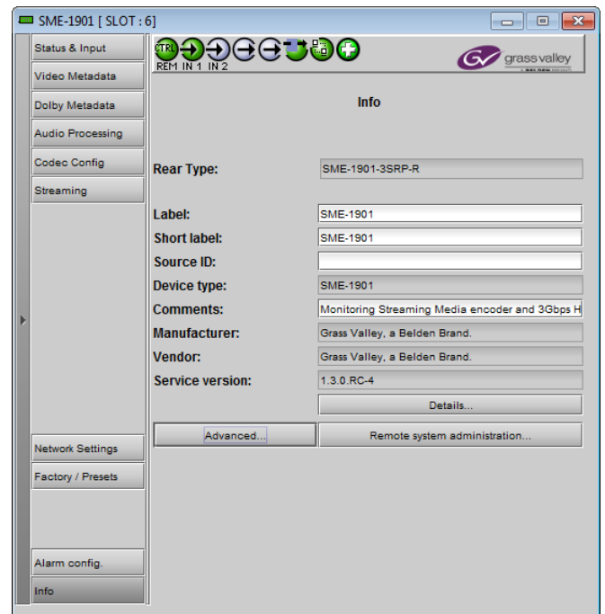
Figure 5-22 Info panel
