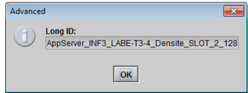
Figure 5-24 Advanced window
