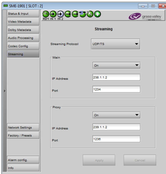
Figure 5-10 Streaming panel
