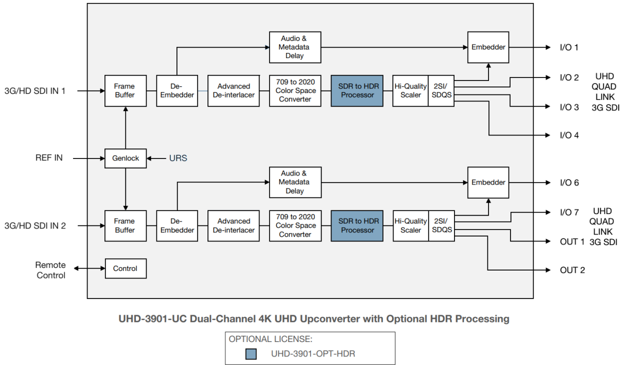
Figure 1-1 UHD-3901 Functional Block Diagram
