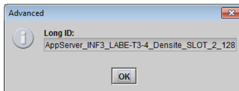
Figure 5-19 Advanced window
