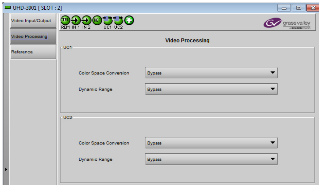
Figure 5-5 Video Processing
