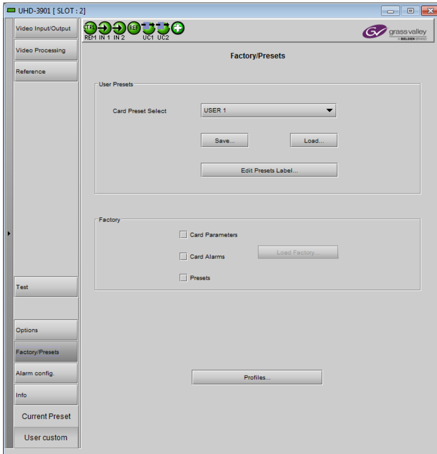
Figure 5-9 Factory/Presets Panel
