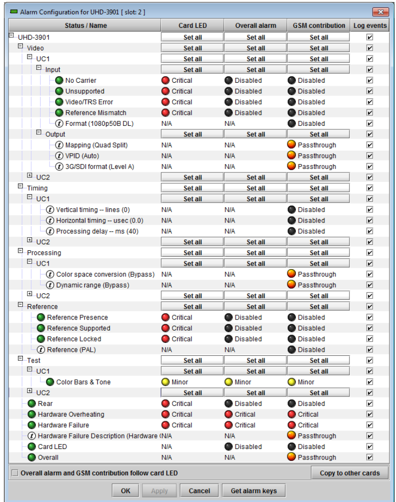
Figure 5-13 Alarm Configuration
