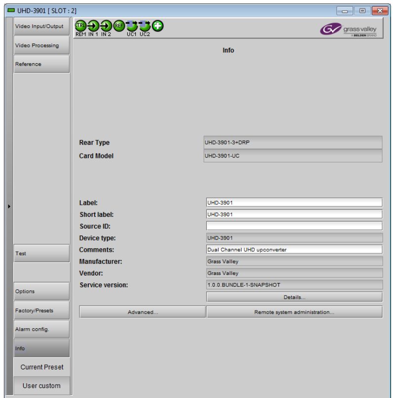
Figure 5-17 Info Panel
