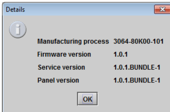
Figure 5-18 Details window
