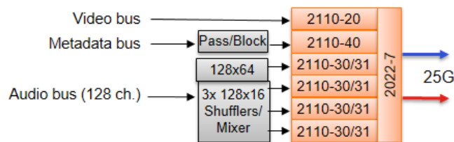
Figure 15 – XIP-3901-UDC-IP / -GB-IP Transmitter Overview
