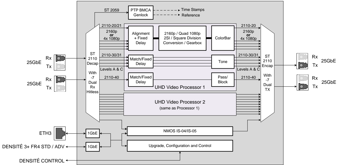
XIP-3901-GB-IP Dual Channel 4K UHD Gearbox IP Processing Application
