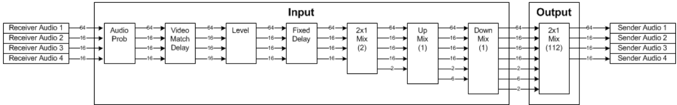
Figure 71 – Overview of XIP-3901-UDC-IP Audio Processing
