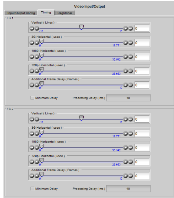
Figure 38 – Video I/O Timing
