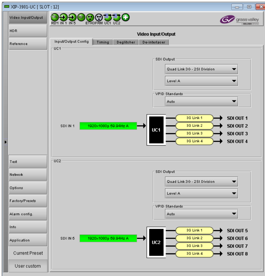
Figure 16 – XIP-3901 iControl Graphic Interface (Shown on XIP-3901-UC)
