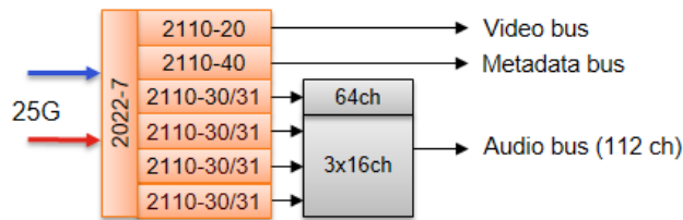
Figure 14 – XIP-3901-UDC-IP / -GB-IP Receiver Overview
