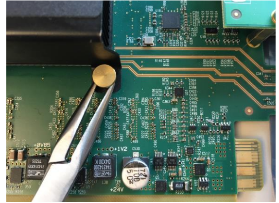
Figure 105 —Prying Out the Pushpins
