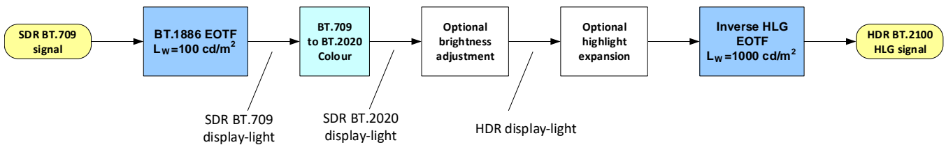
Figure 110 – SDR to HDR Display-Light Conversion
