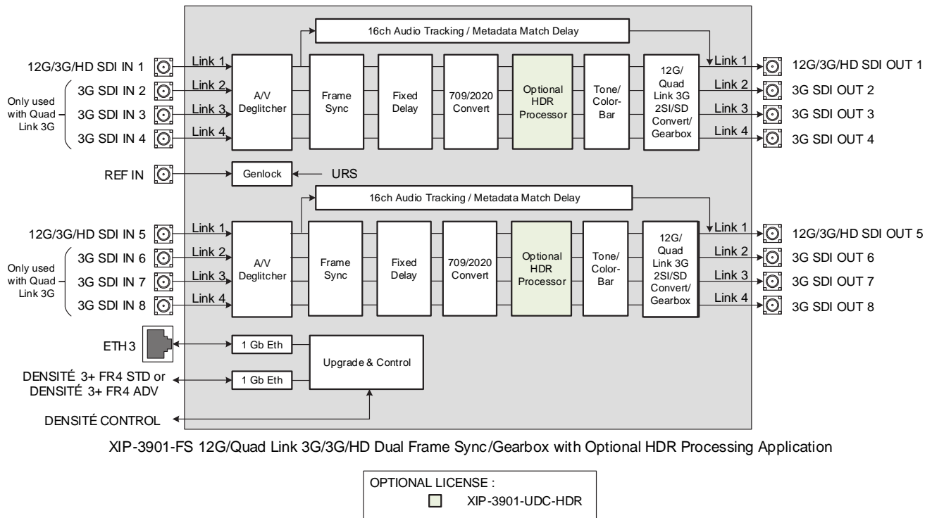
Figure 6–XIP-3901-FS Functional Block Diagram
