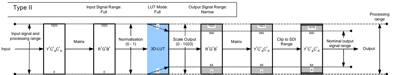
Figure 108 – Type II signal scaling, intended for full-range input signals (for example, S-Log3)
