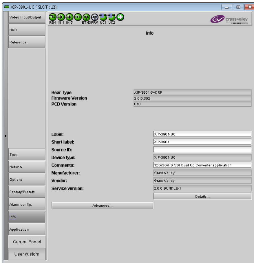
Figure 97 – Info Panel (Shown on XIP-3901-UC)
