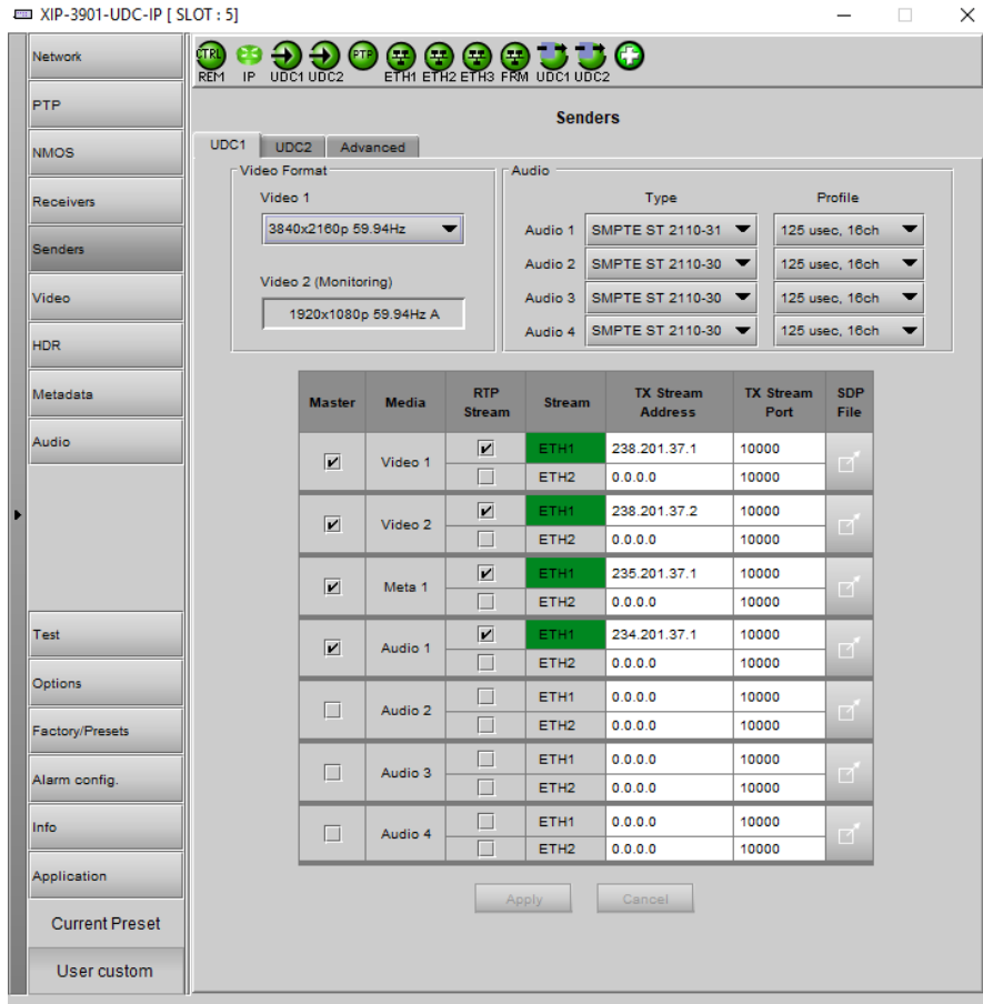
Figure 60 – Senders UDC1 Tab
