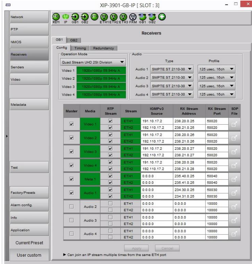
Figure 80 – Receivers Config Tab
