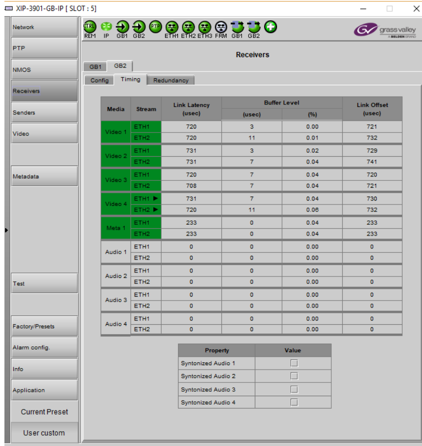
Figure 81 – Receivers Timing Tab
