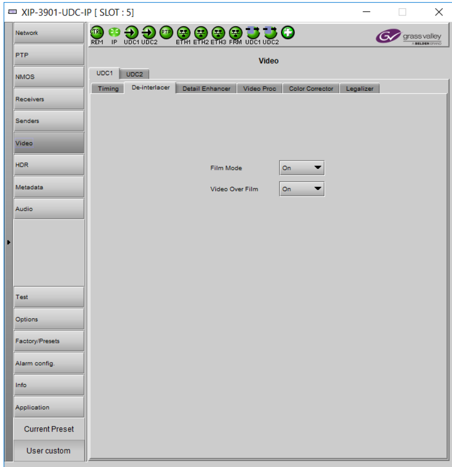
Figure 64 – De-interlacer Timing Tab
