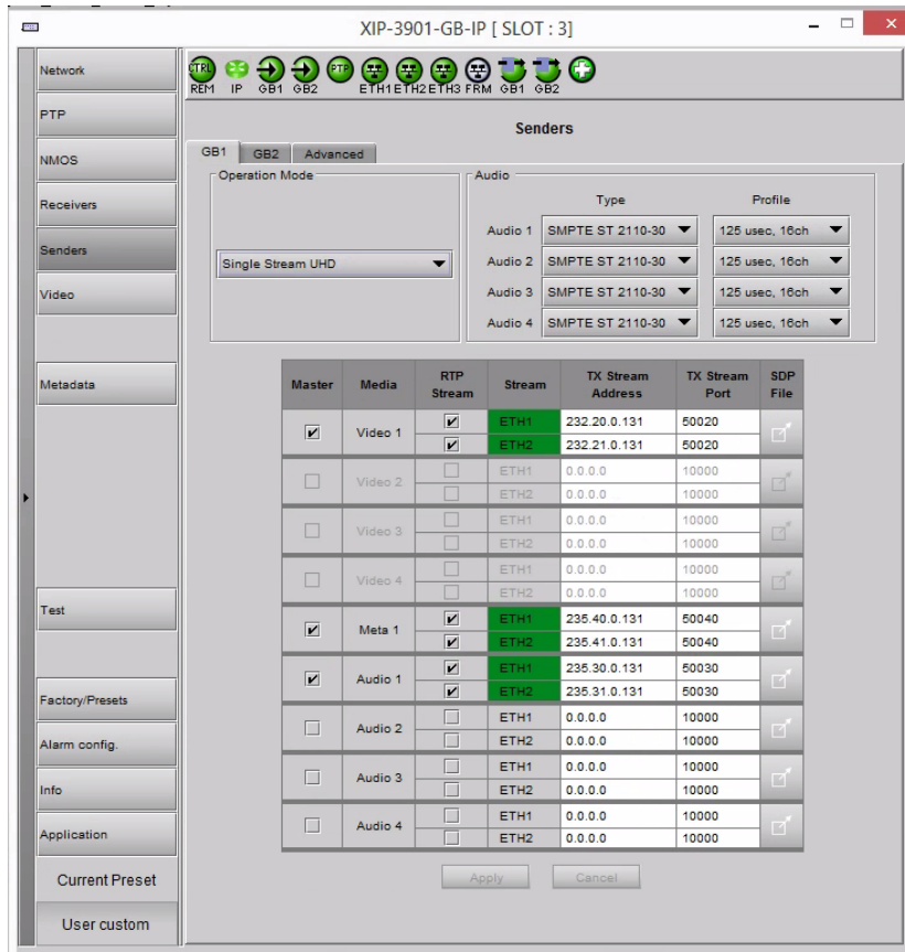
Figure 82 – Senders GB1 / GB2 Tab
