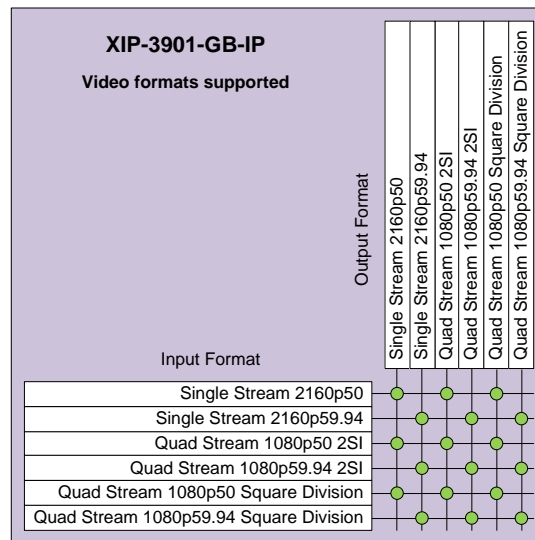
Figure 9 —Supported Video Formats for XIP-3901-GB-IP Applications
