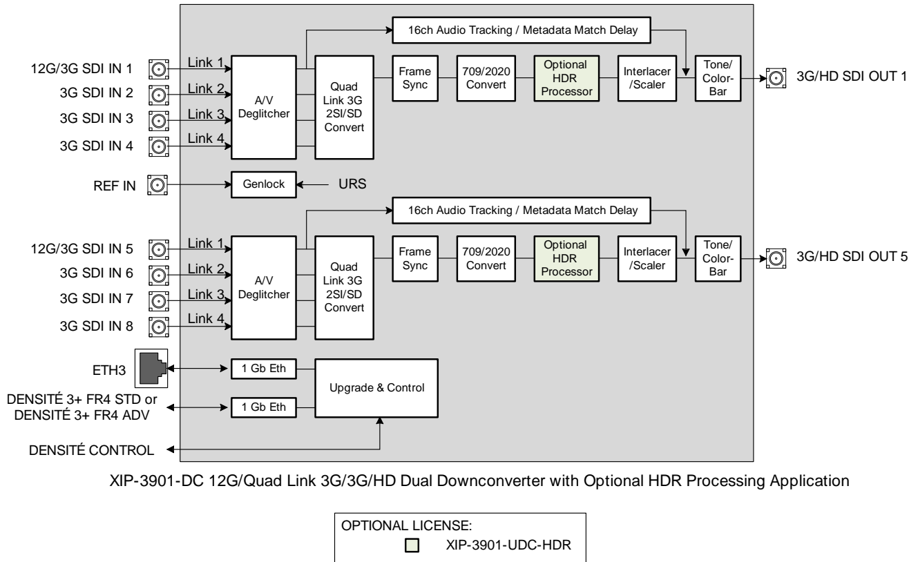
Figure 5–XIP-3901-DC Functional Block Diagram
