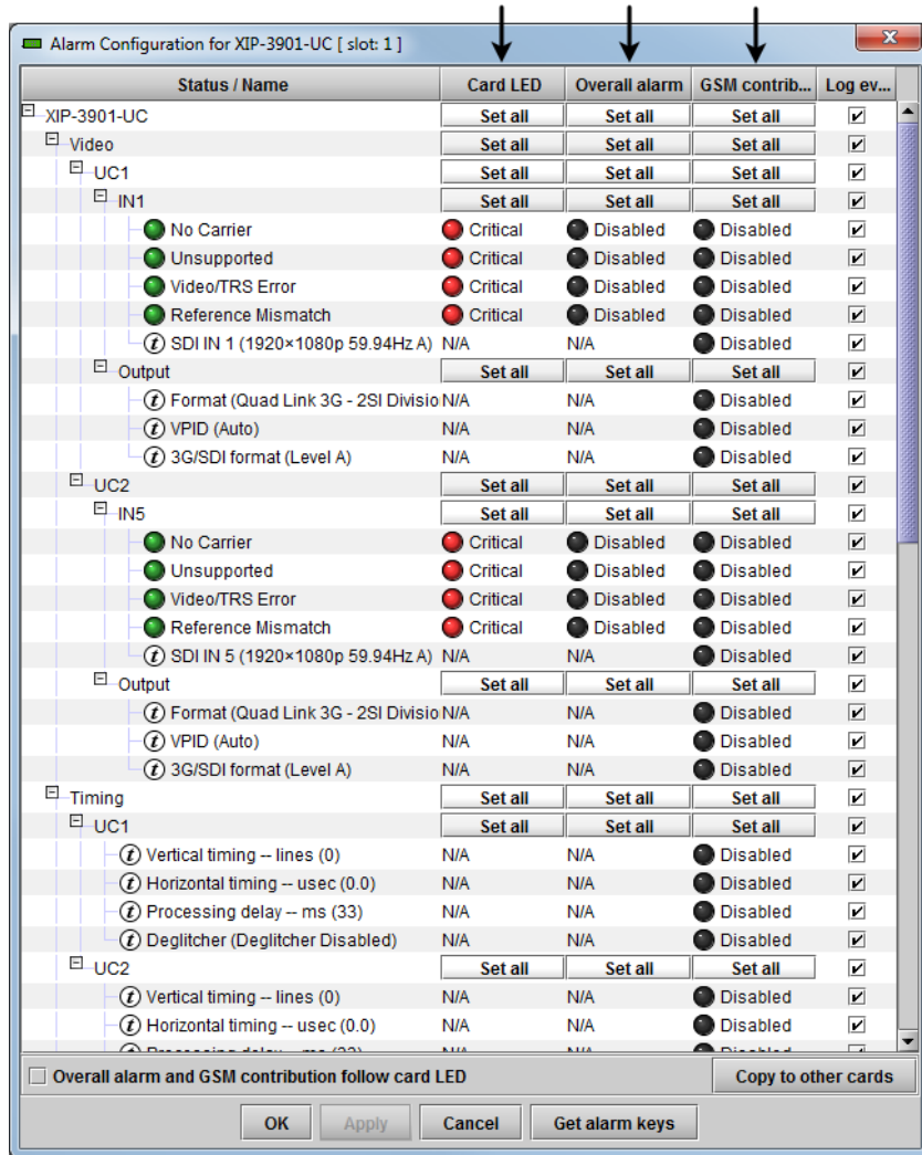
Figure 88—Alarm Types Reset by Load Factory (Shown on XIP-3901-UC)
