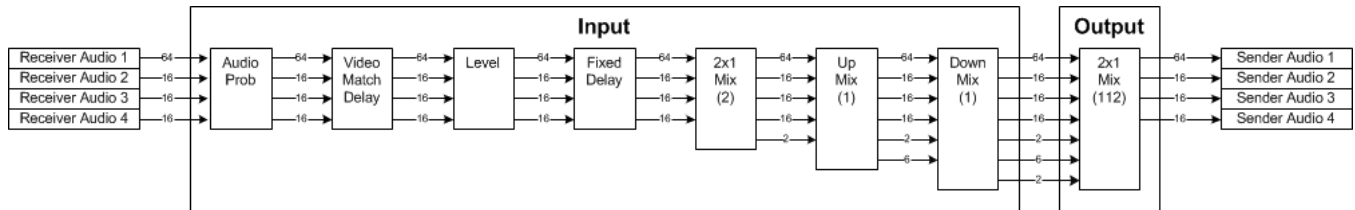
Figure 72 – Overview of XIP-3901-UDC-IP Audio Processing
