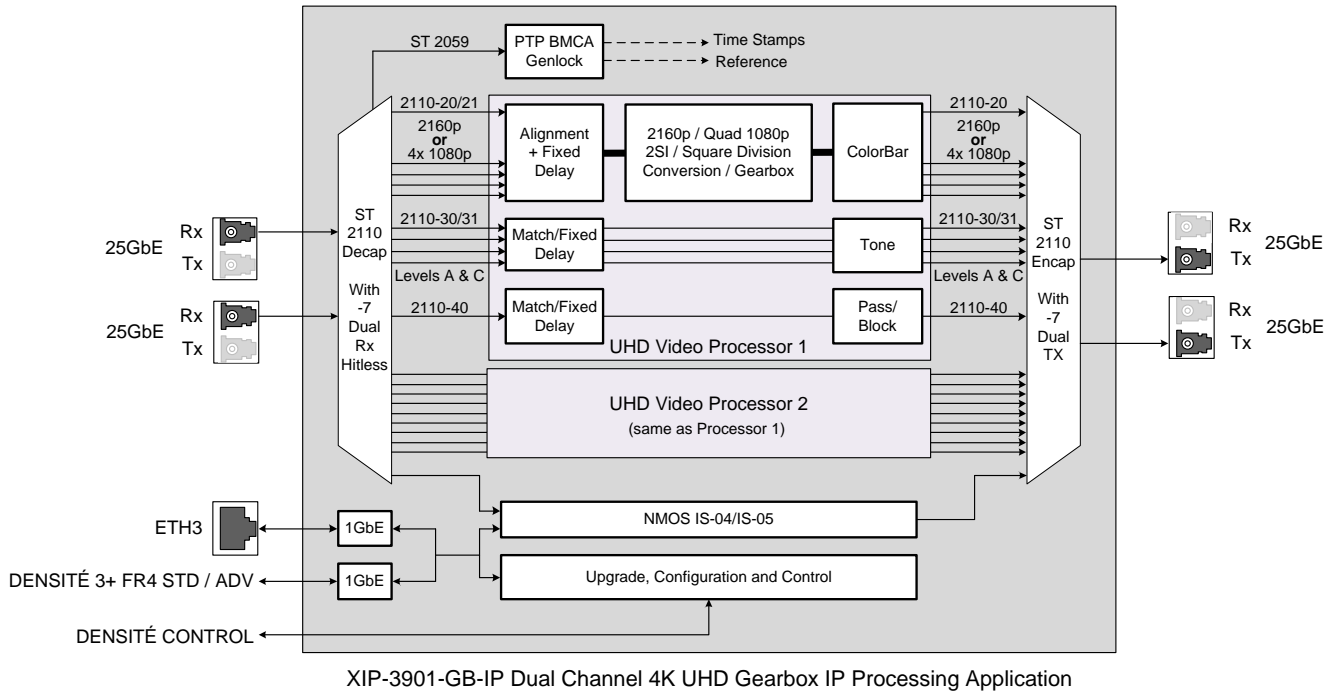
Figure 10 – XIP-3901-GB-IP Functional Block Diagram
