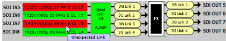
Figure 37—Synchronization Diagram
