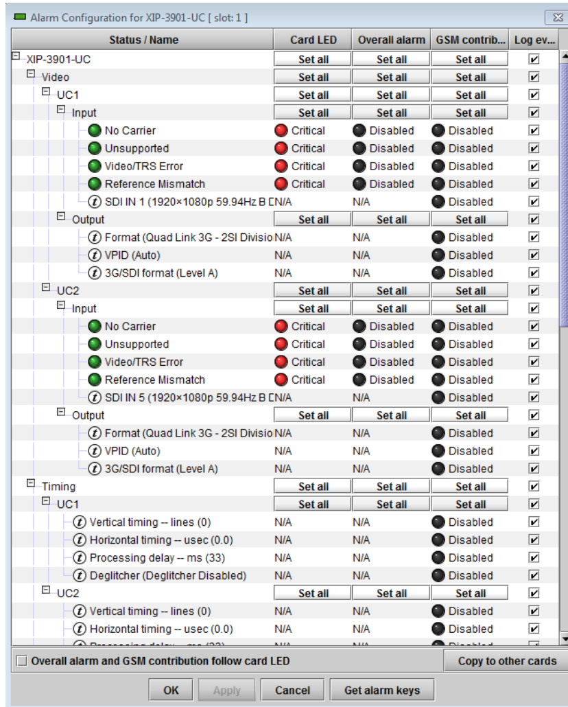
Figure 93—Alarm Configuration (Shown on XIP-3901-UC)
