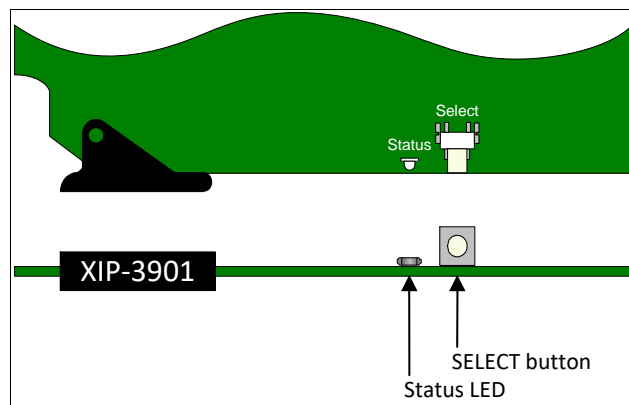
Figure 12 –Front Card-edge Layout
