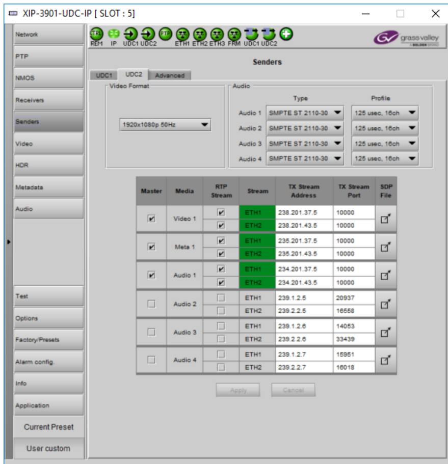
Figure 61 – Senders UDC2 Tab
