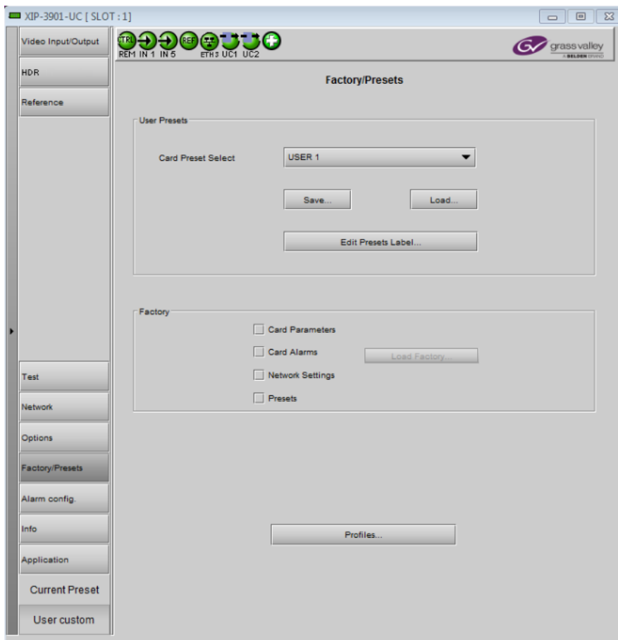
Figure 84 – Factory/Presets Panel (Shown on XIP-3901-UC)
