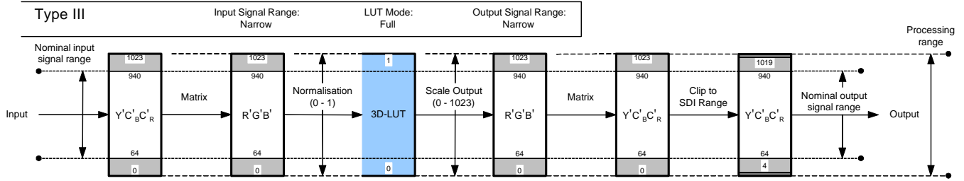
Figure 109 – Type III signal scaling, primarily intended for hardware-based LUT applications
