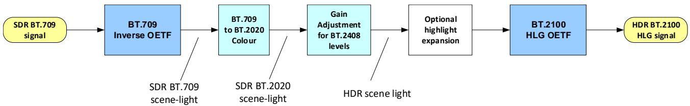
Figure 111 – Scene-light SDR to HDR conversion
