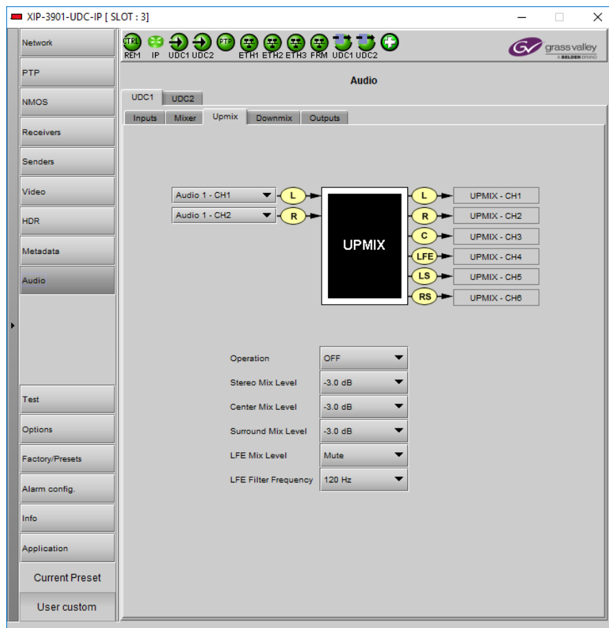
Figure 75 – Audio Upmix Tab
