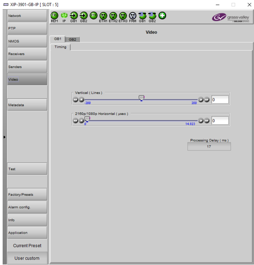
Figure 83 – Video Timing Tab
