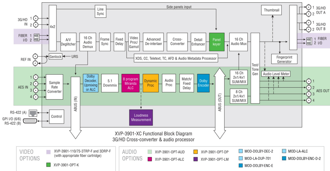
Figure 1.6 Functional block diagram XVP-3901-XC
