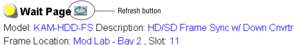
Figure 28. Wait Page
