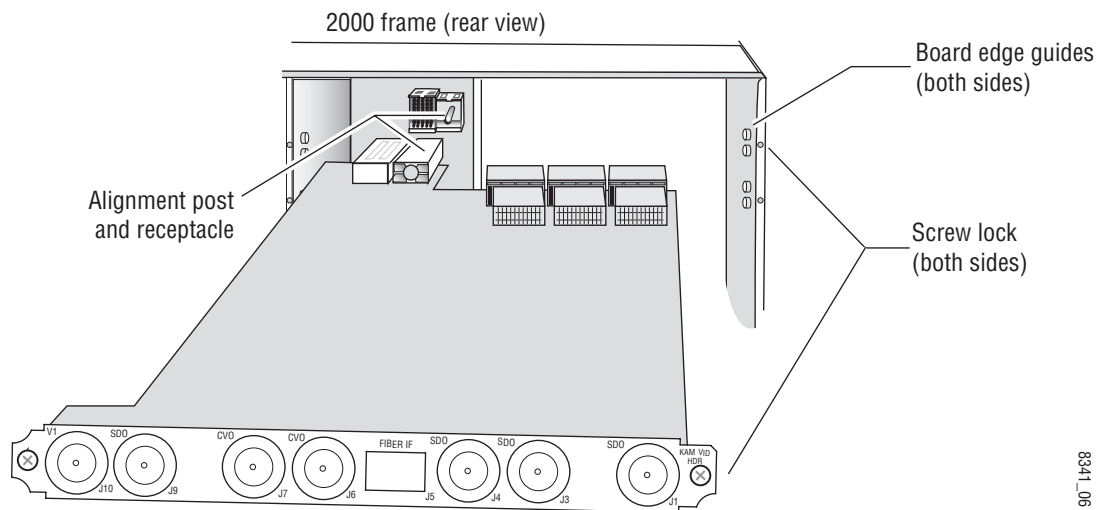
Figure 3. Installing Passive Rear Module
