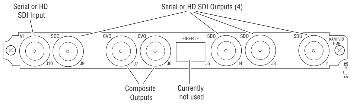
Figure 7. KAM-HD-R Input/Output Connectors
