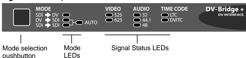
Figure 3.1 Front panel
