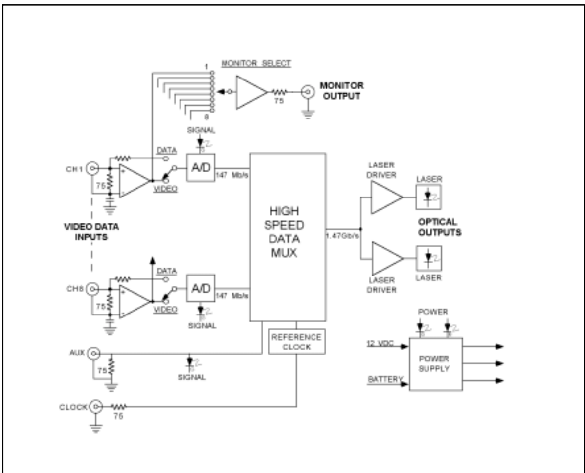
Figure 5. TX Block Diagram
