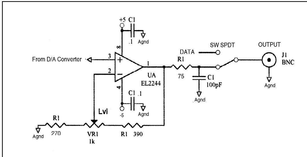
Figure 8. RX Output Schematic
