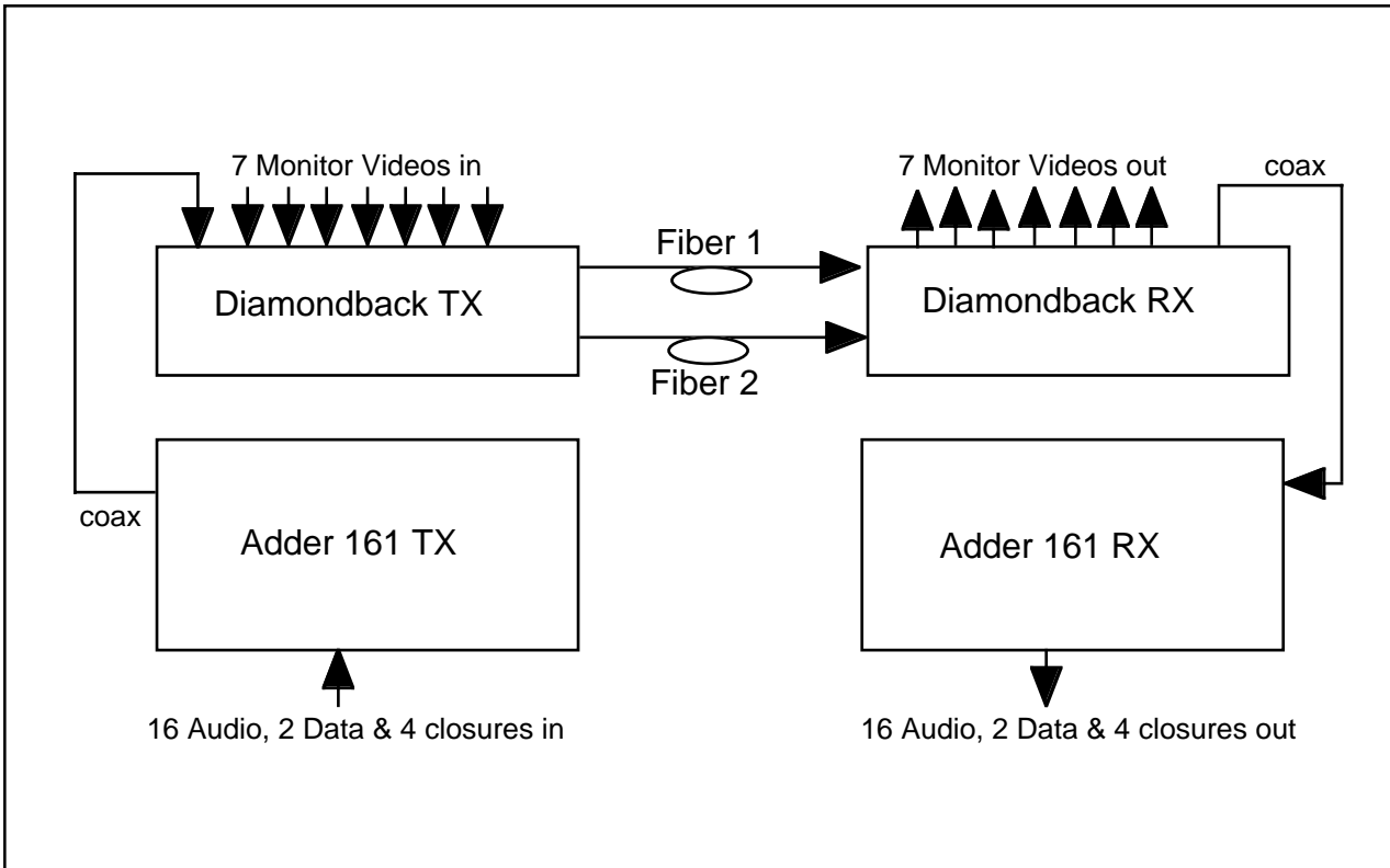
Figure 4. Example of the DiamondBack/Adder 161 Network
