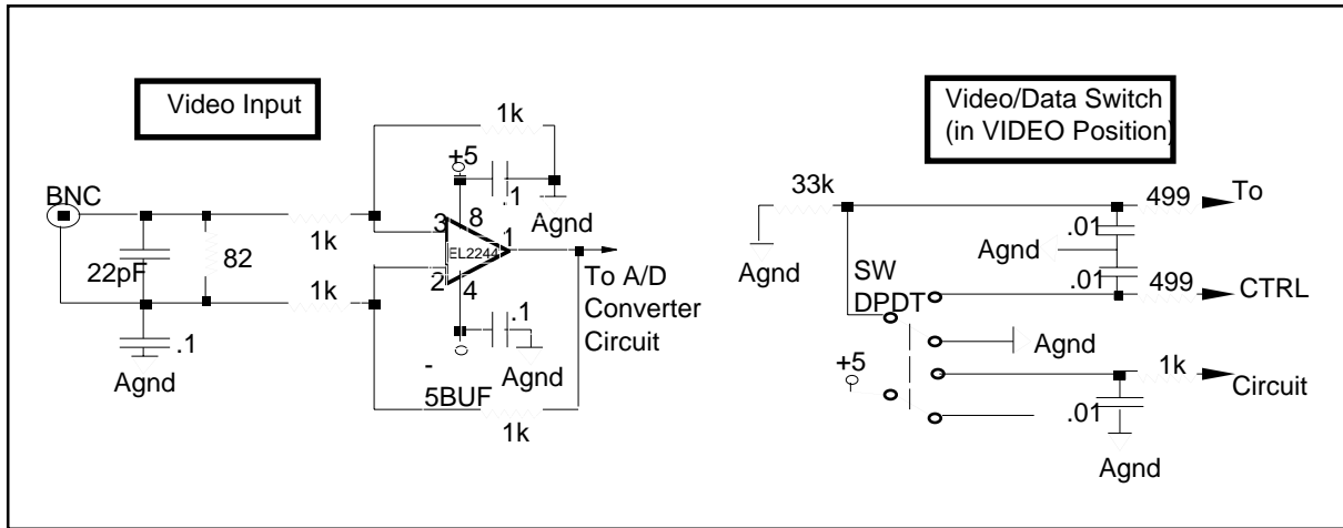
Figure 6. TX Input Schematic
