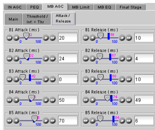
Figure 6-15 ALC - MB-AGC - Attack/Release
