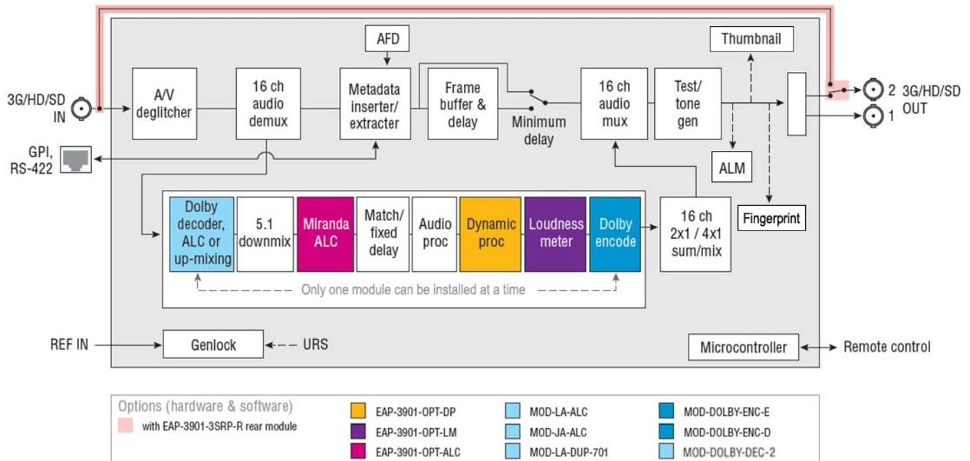
Figure 1.1 EAP-3901 Functional Block Diagram
