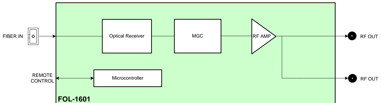
FOL-1601 Functional Block Diagram
