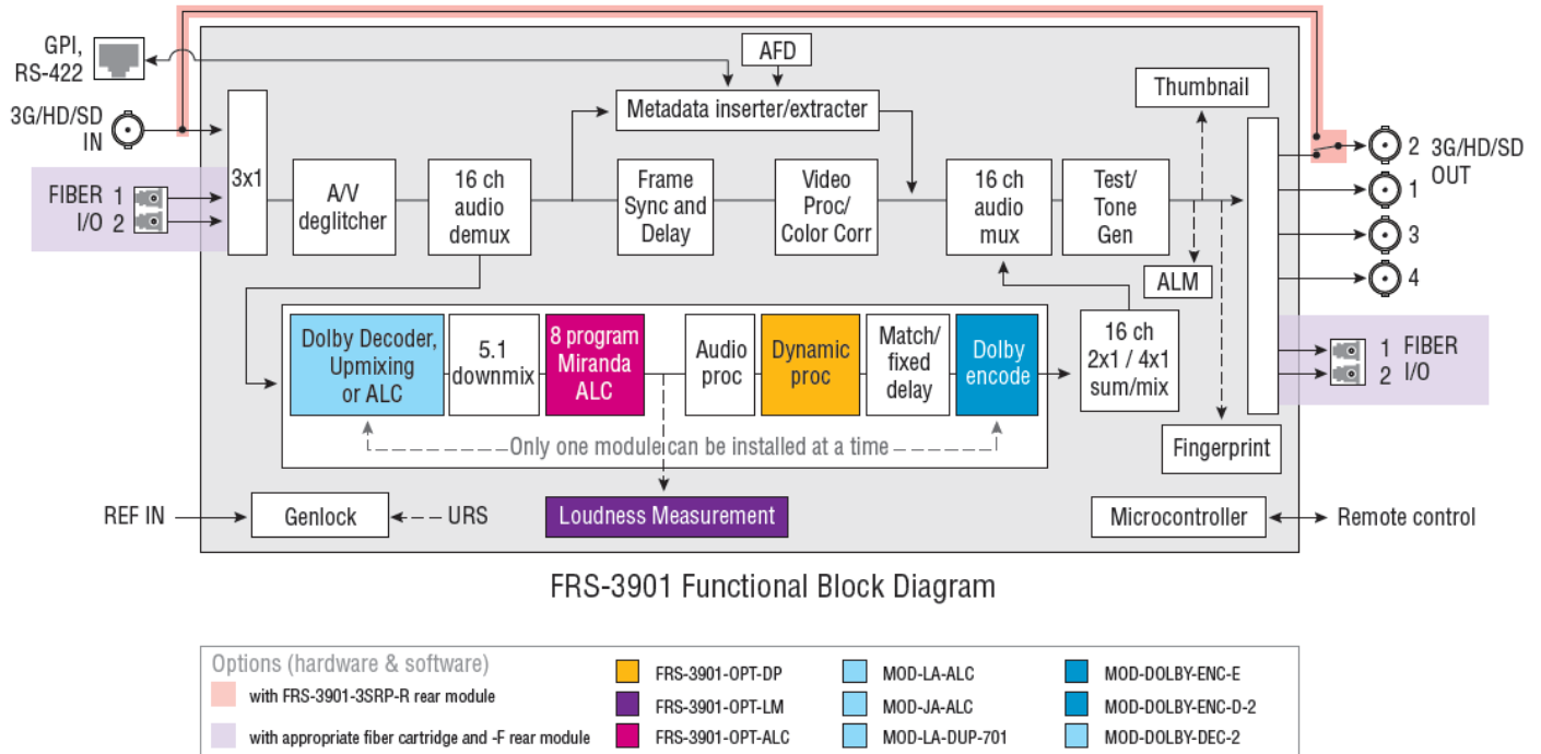
Figure 1.1 FRS-3901 Functional Block Diagram
