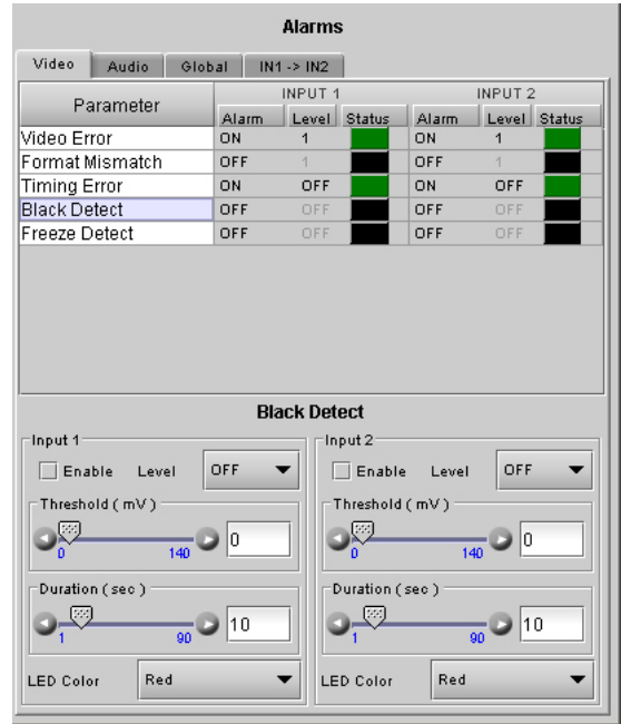
Figure 3.13 Black Detect alarm Config.
