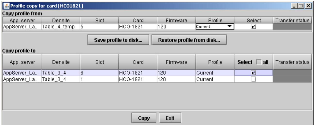
Figure 3.39 Profile copy window
