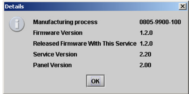
Figure 3.35 Details window
