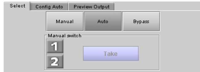
Figure 3.6 Auto Mode
