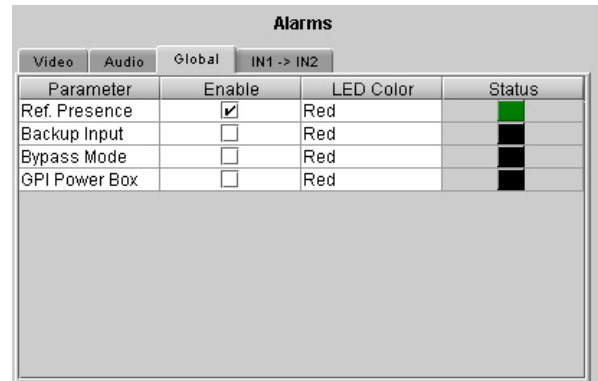
Figure 3.17 Global alarms
