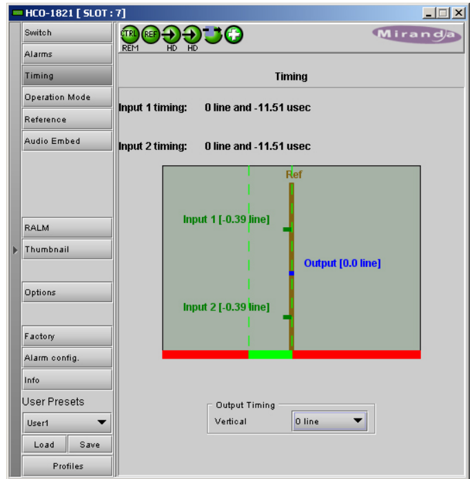
Figure 3.20 Timing panel
