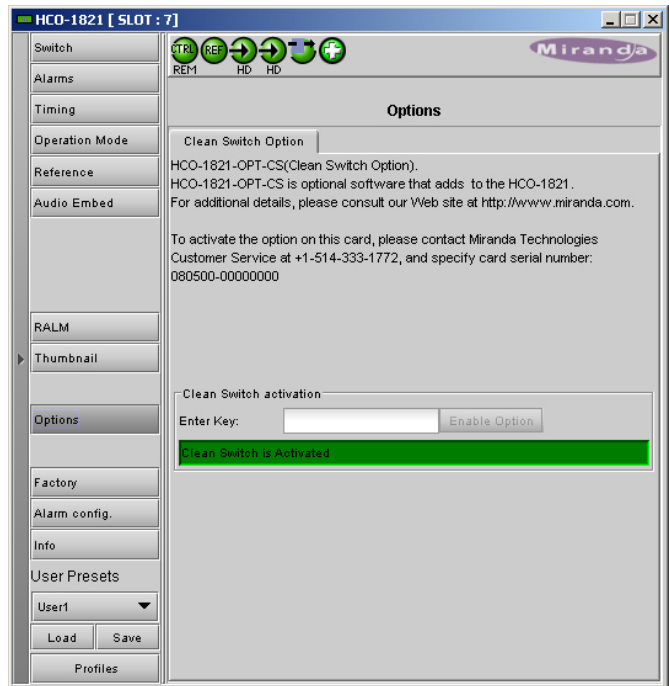
Figure 3.29 Options Panel
