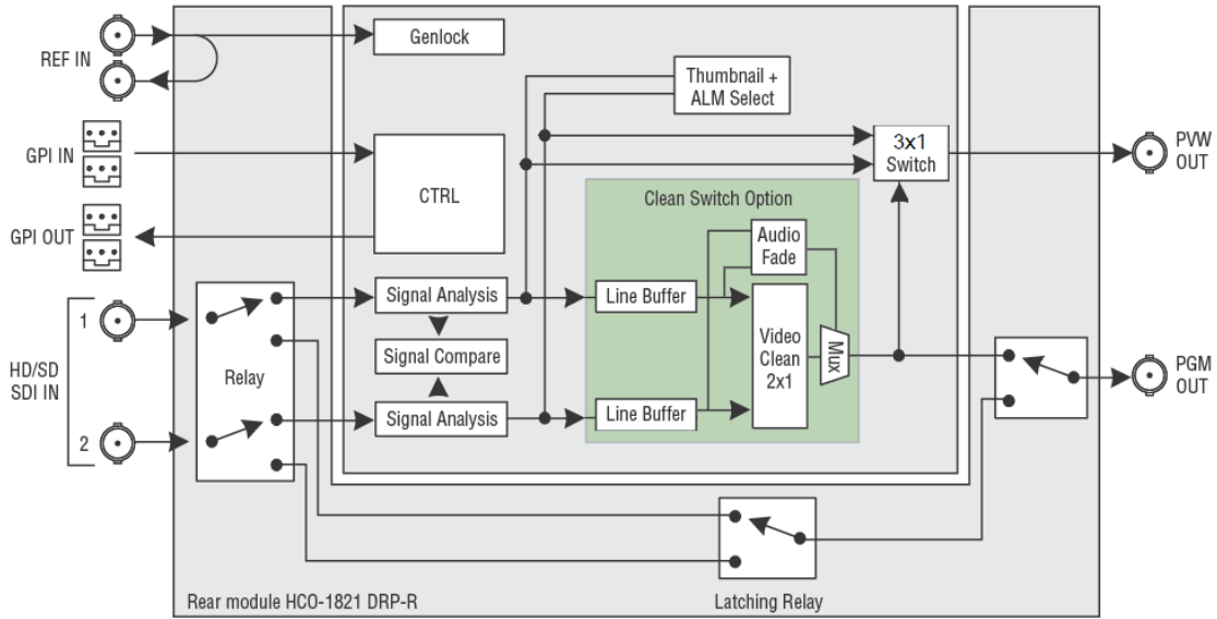
Figure 1.1 Functional block diagram HCO-1821
