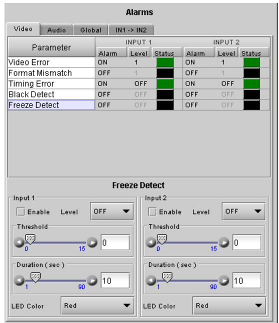
Figure 3.14 Freeze Detect alarm Config.
