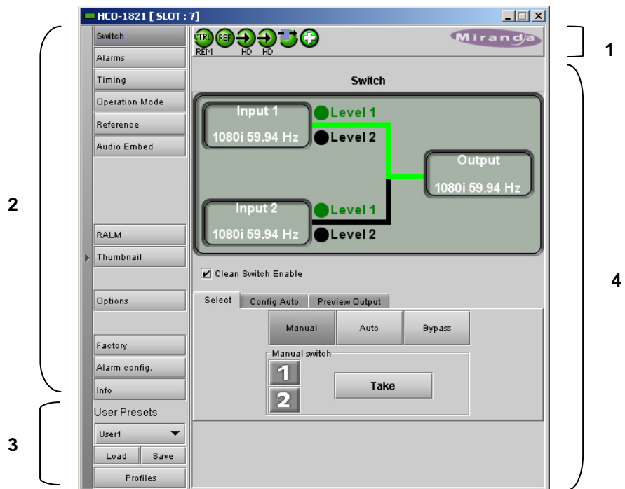
Figure 3.2 HCO-1821 iControl graphic interface window
