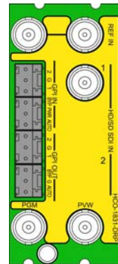
Figure 2.1 HCO-1821 Rear Panel
