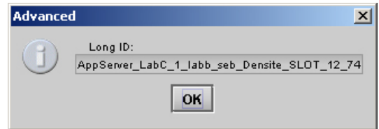
Figure 3.36 Advanced window
