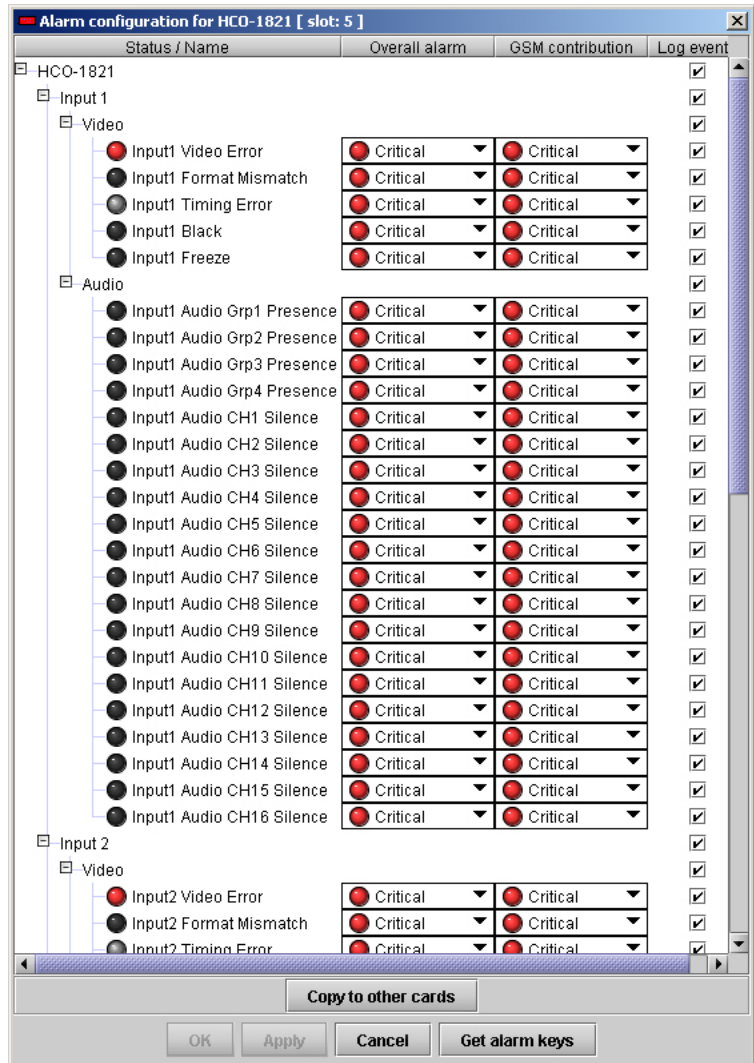
Figure 3.31 Alarm Configuration Panel
