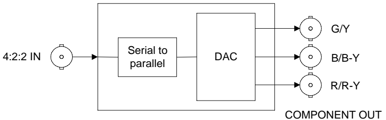
Figure 1: SDM-171p functional block diagram
