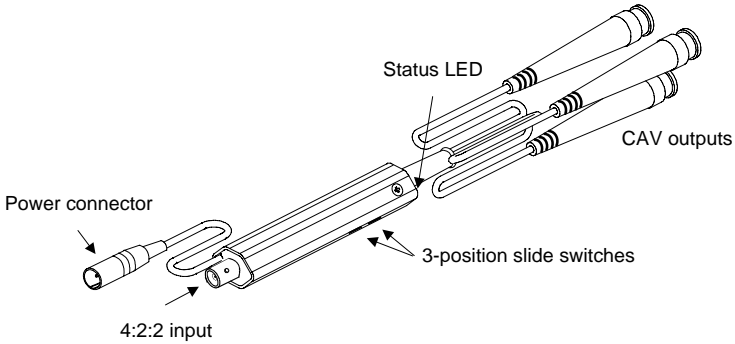
Figure 2: Physical layout of the SDM-171p
