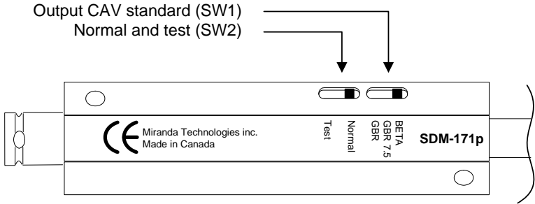
Figure 4: SDM-171p switch settings
