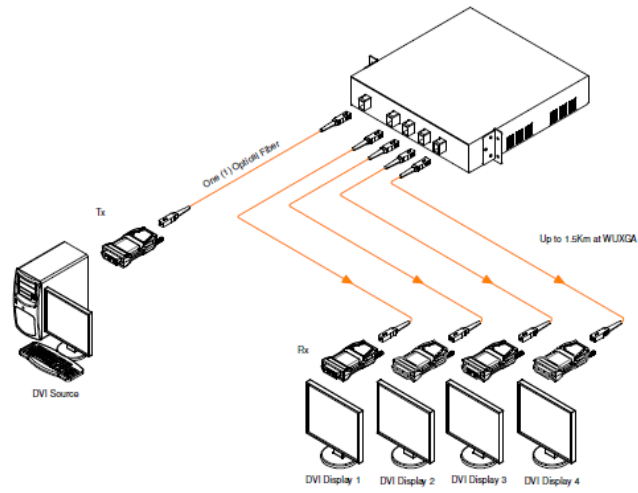
Figure 5 – Connection diagram using optical splitter.
