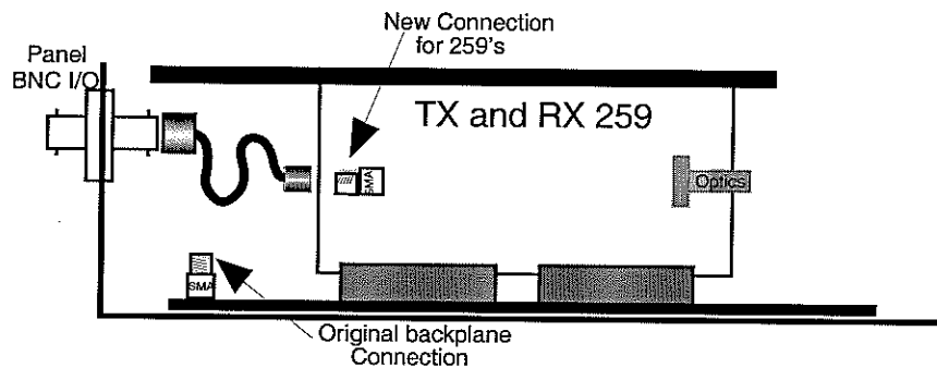
Figure 24. TX/RX 259 Connections
