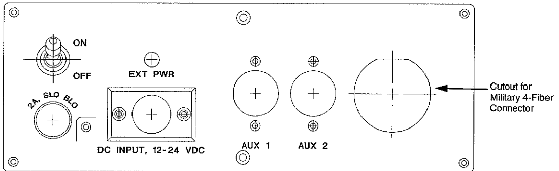
Figure 8. VIM4 Front Panel
