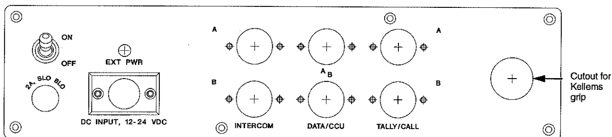
Figure 10. VIM8 Front Panel
