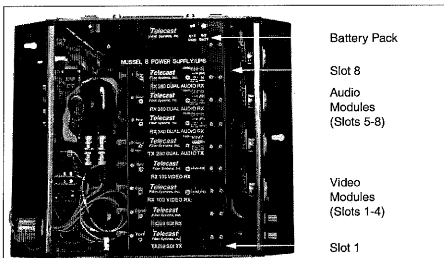
Figure 46. 8-Slot Configuration
