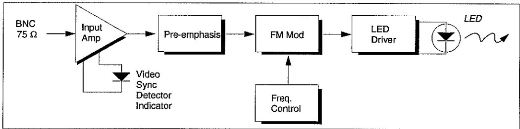
Figure 19. Analog Video Input Schematic
