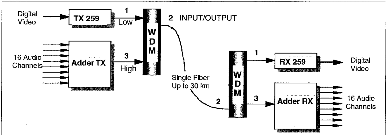
Figure 4. WDM Application
