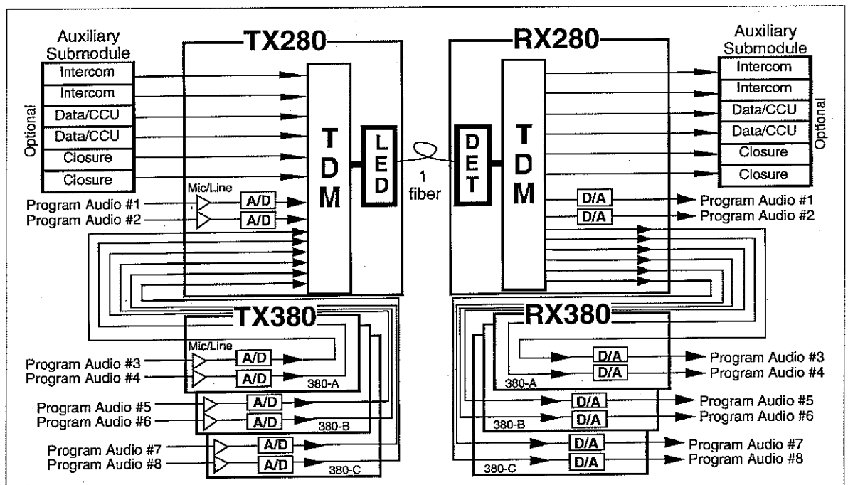
Figure 31. TX/RX 280 and 380 Module Sets Block Diagram
