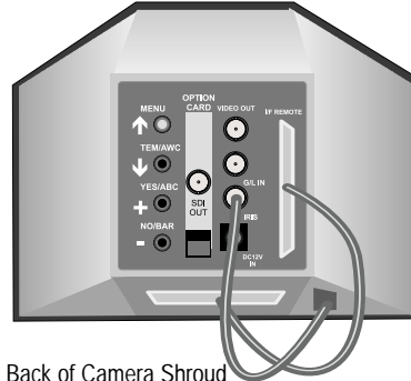
Back of Camera Shroud
