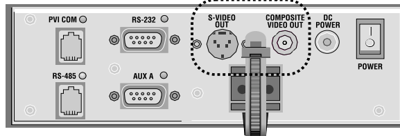
Ports and Jacks
