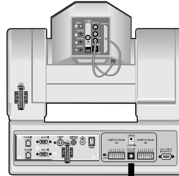
Back of 3-CCD DIGITAL Camera
