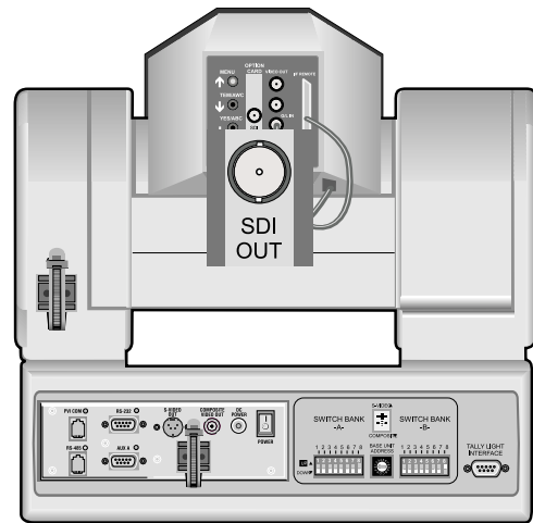
Back of 3-CCD CameraMan with configuration plate removed
