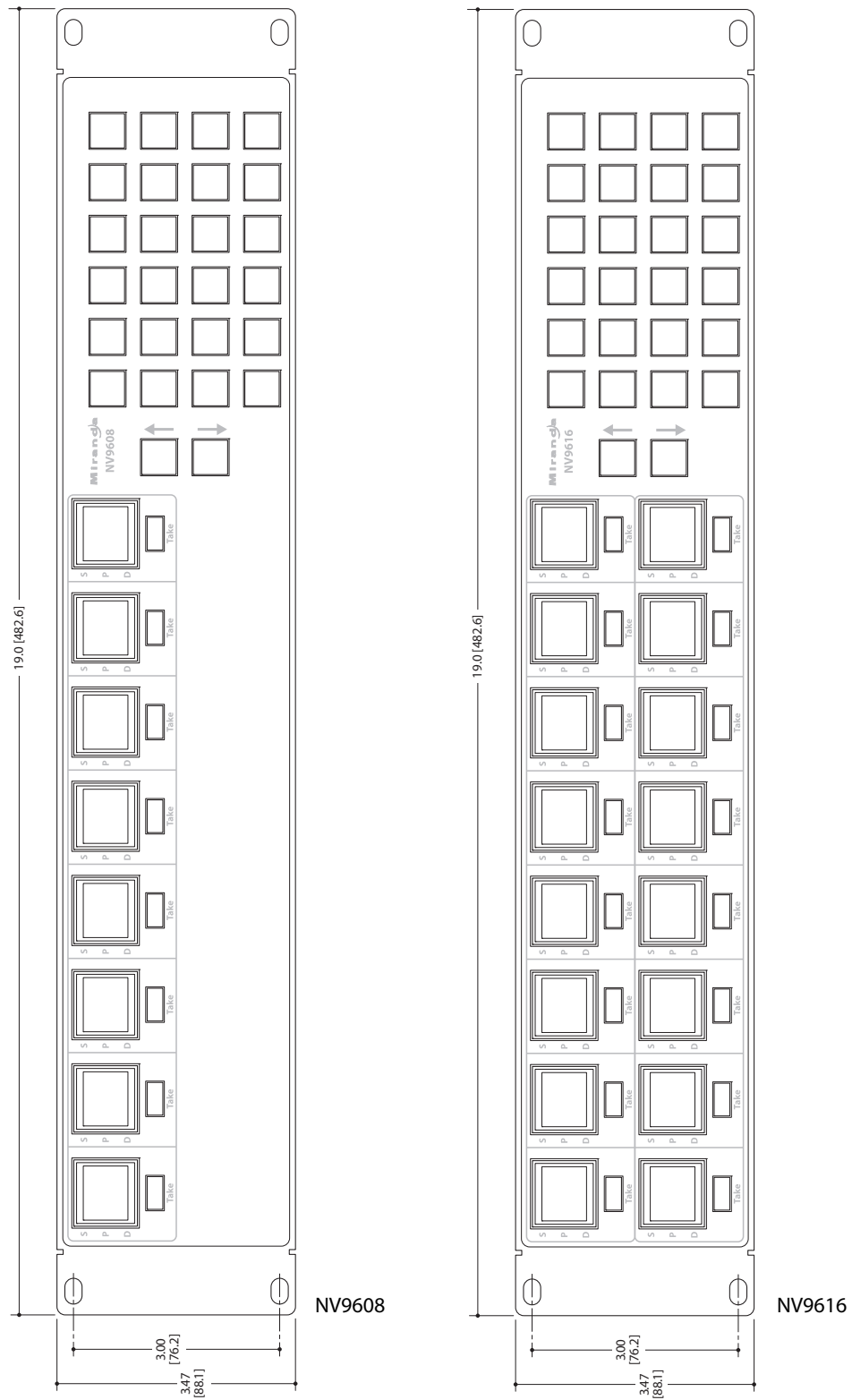
Fig. 6-2: Front Views of the NV9608 and NV9616
