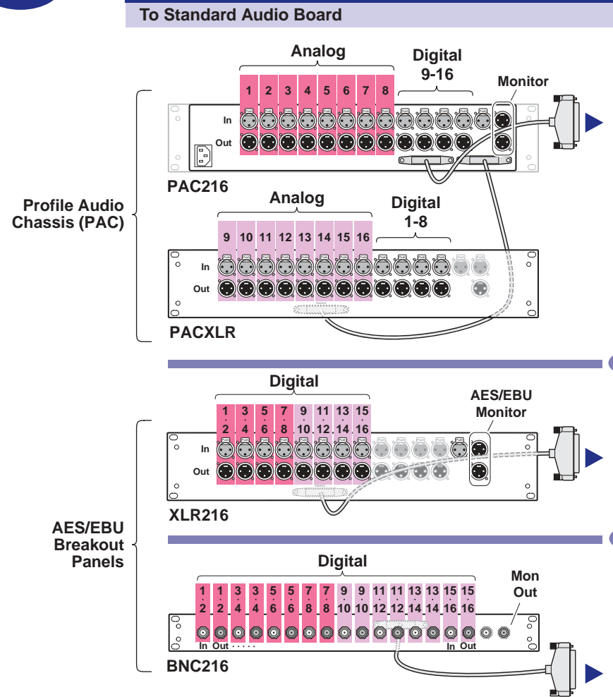
Audio I/O Connections: Two Audio Boards Installed
