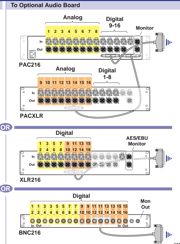
Audio I/O Connections: Two Audio Boards Installed
