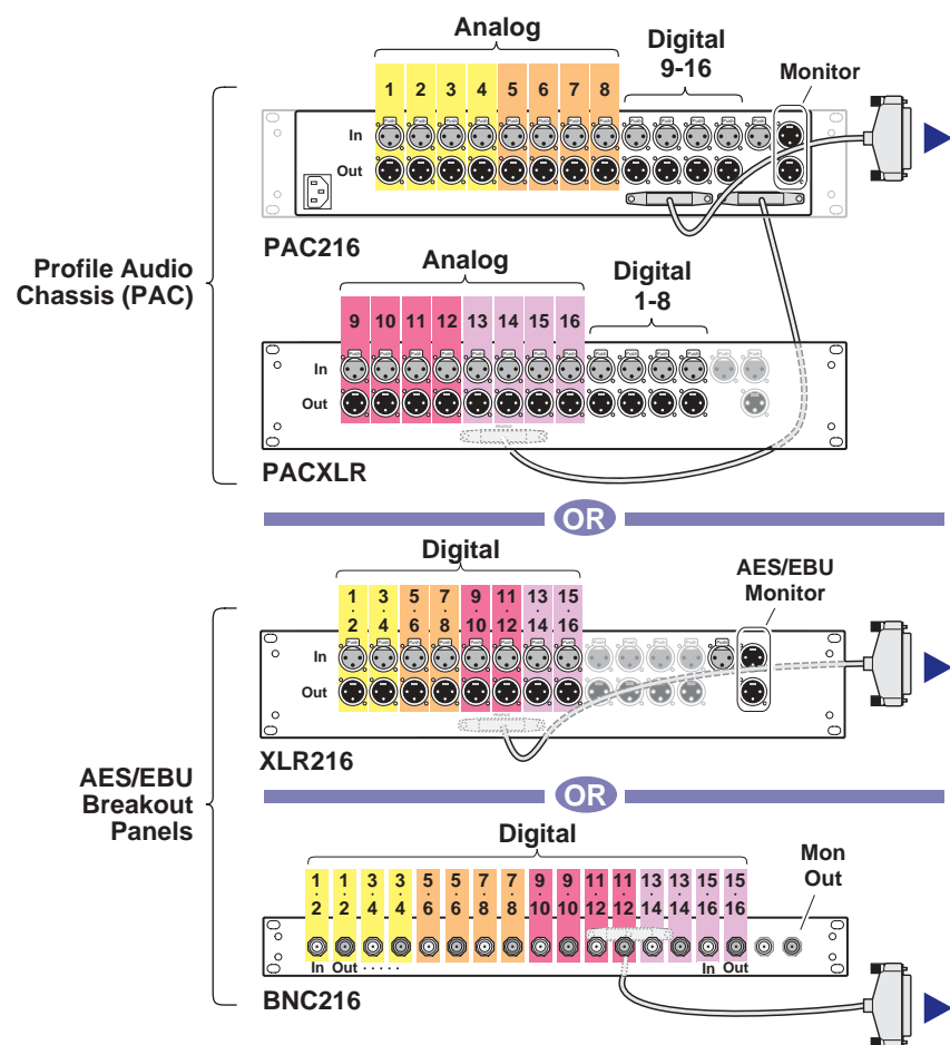
Audio I/O Connections: One Audio Board Installed
