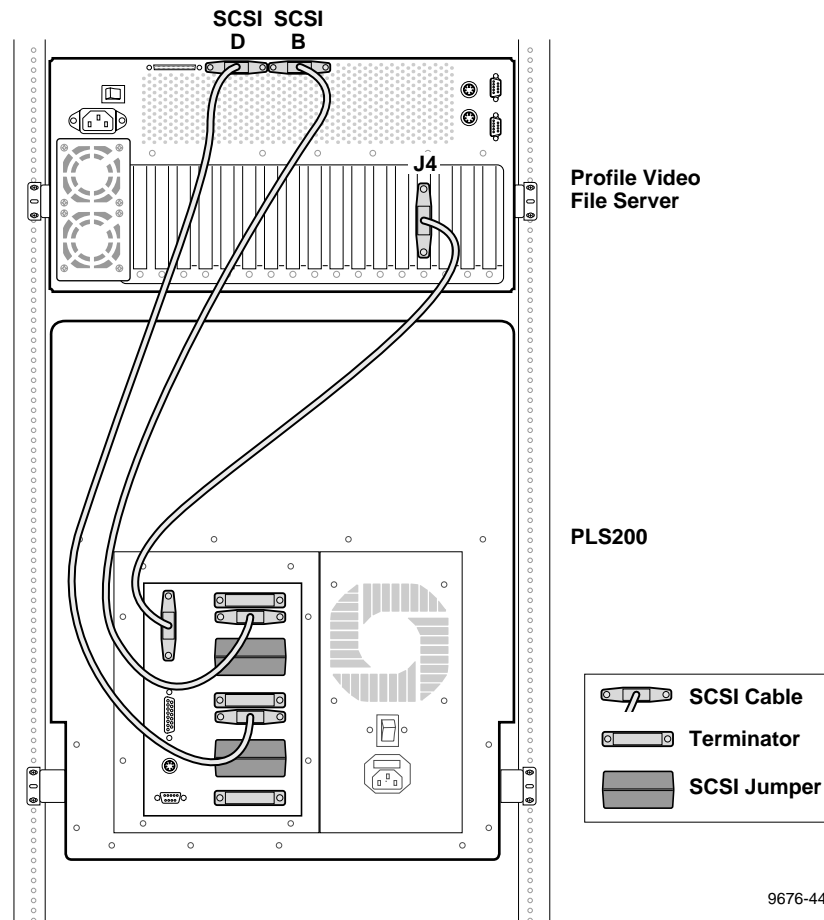
Figure 2-23. Example 3: Profile Video File Server to PLS 200 Connections
