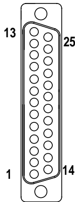
Figure B-7. Reference Genlock 25-pin Connector
