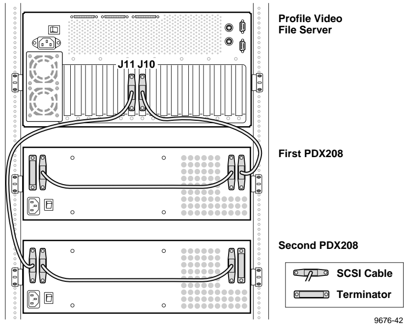
Figure 2-22. Example 2: Profile Video File Server to Two PDX 208 Disk Expansion Connections
