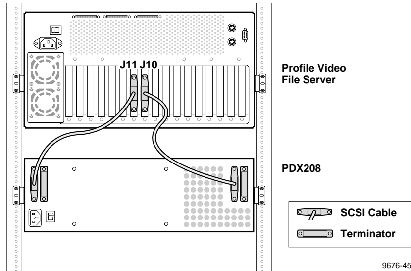
Figure 2-21. Example 1: Profile Video File Server to PDX 208 Disk Expansion Connections
