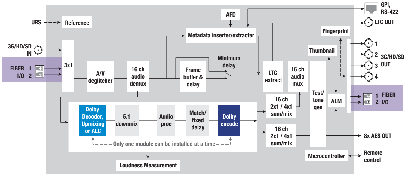
ADX-3981 Functional Block Diagram
