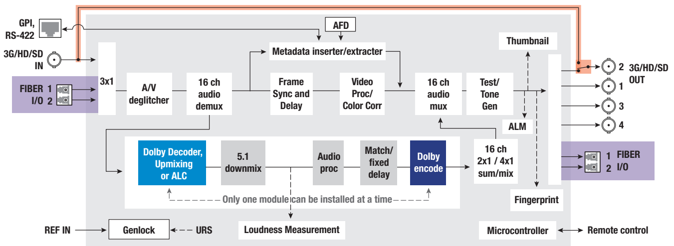
FRS-3901 Functional Block Diagram
