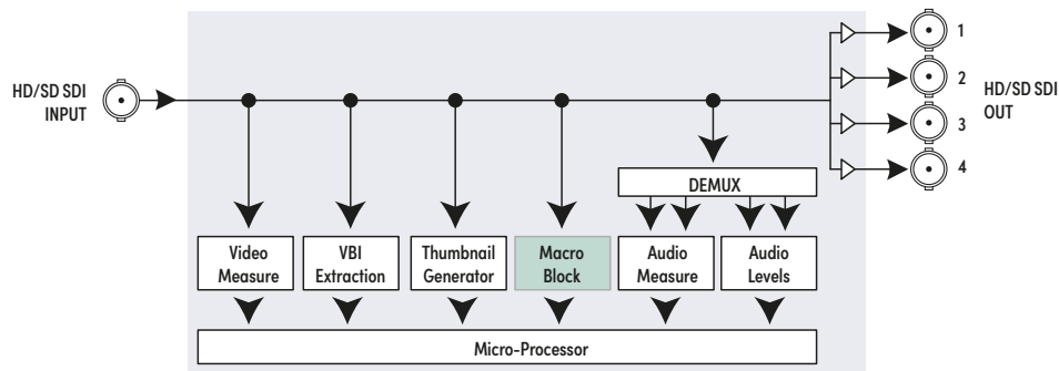
HCP-1801 Functional Block Diagram
